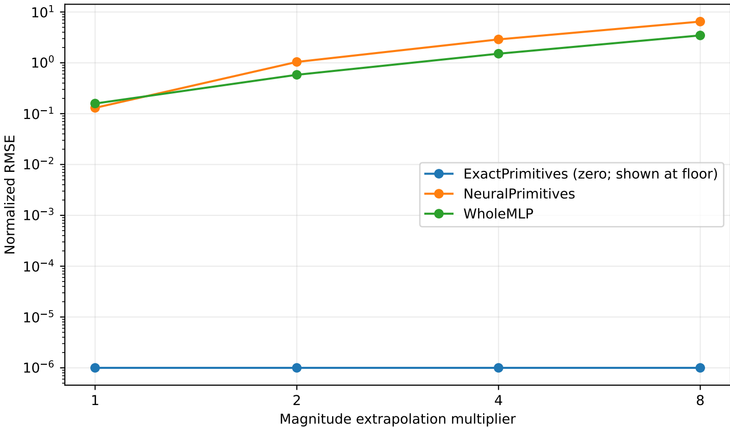
Same oracle graph: exact vs neural primitive execution
