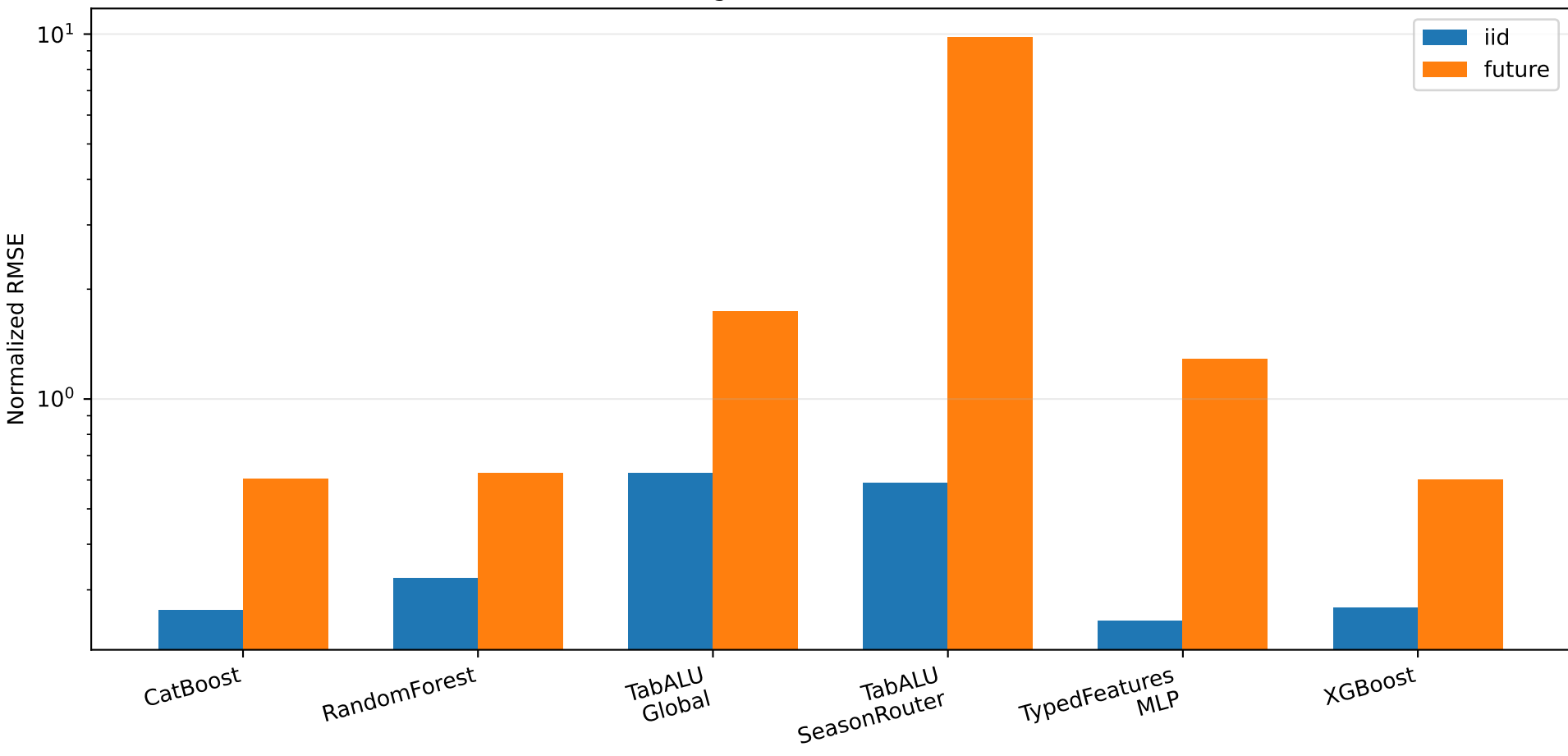
UCI Bike Sharing: 2011 IID holdout vs all of 2012
