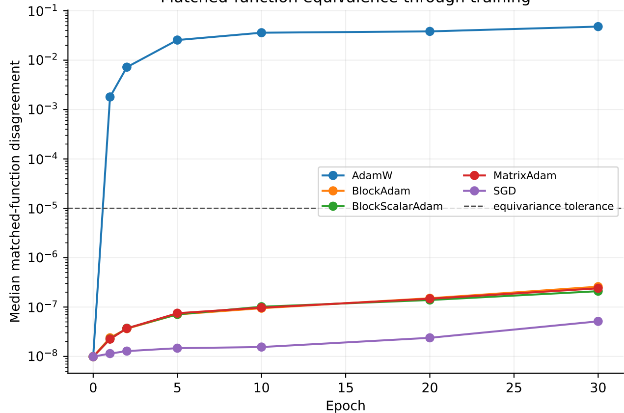
Matched-function equivalence through training
