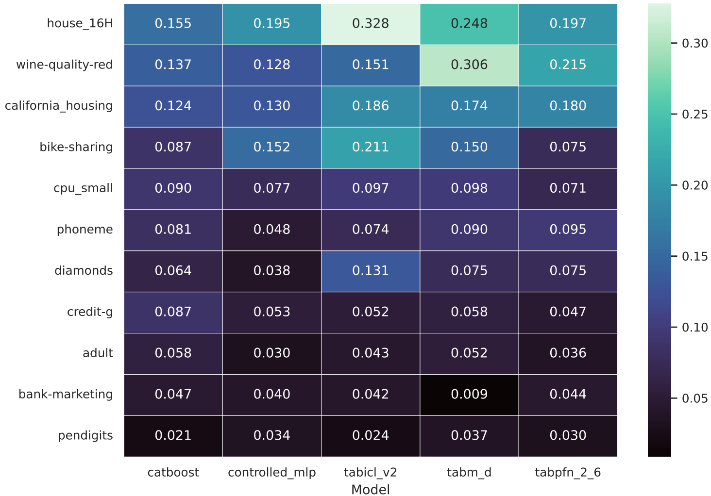
Orthogonal all-block prediction disagreement
