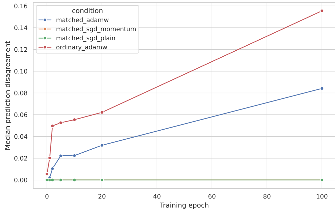
Function matching and optimizer geometry
