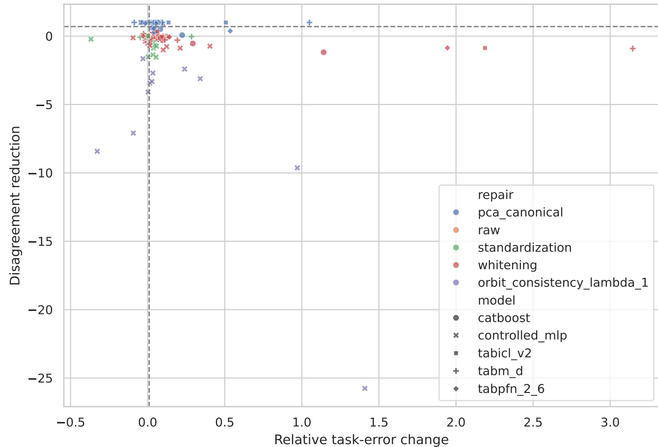
Task performance-invariance tradeoff
