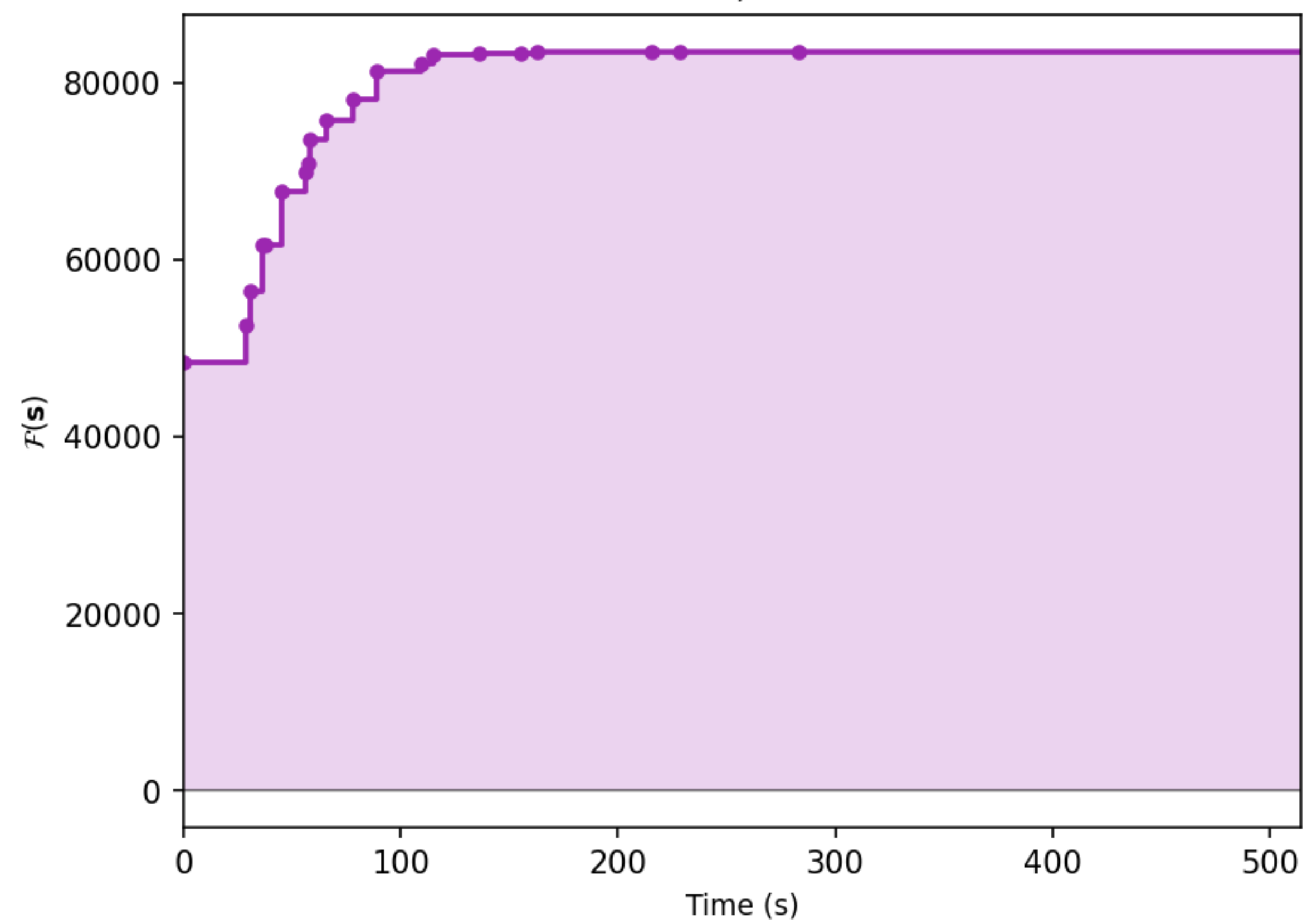
Variable=15800, clauses=48478
