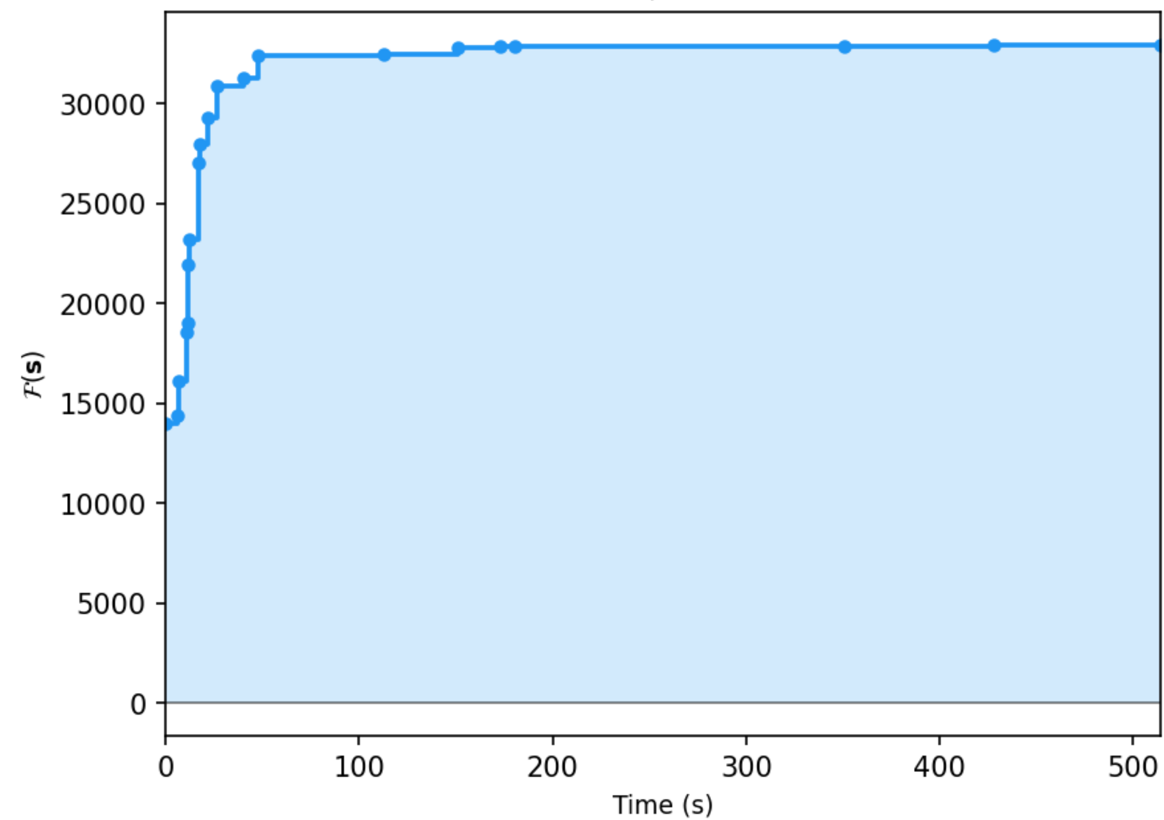
Variable=11850, clauses=36296
