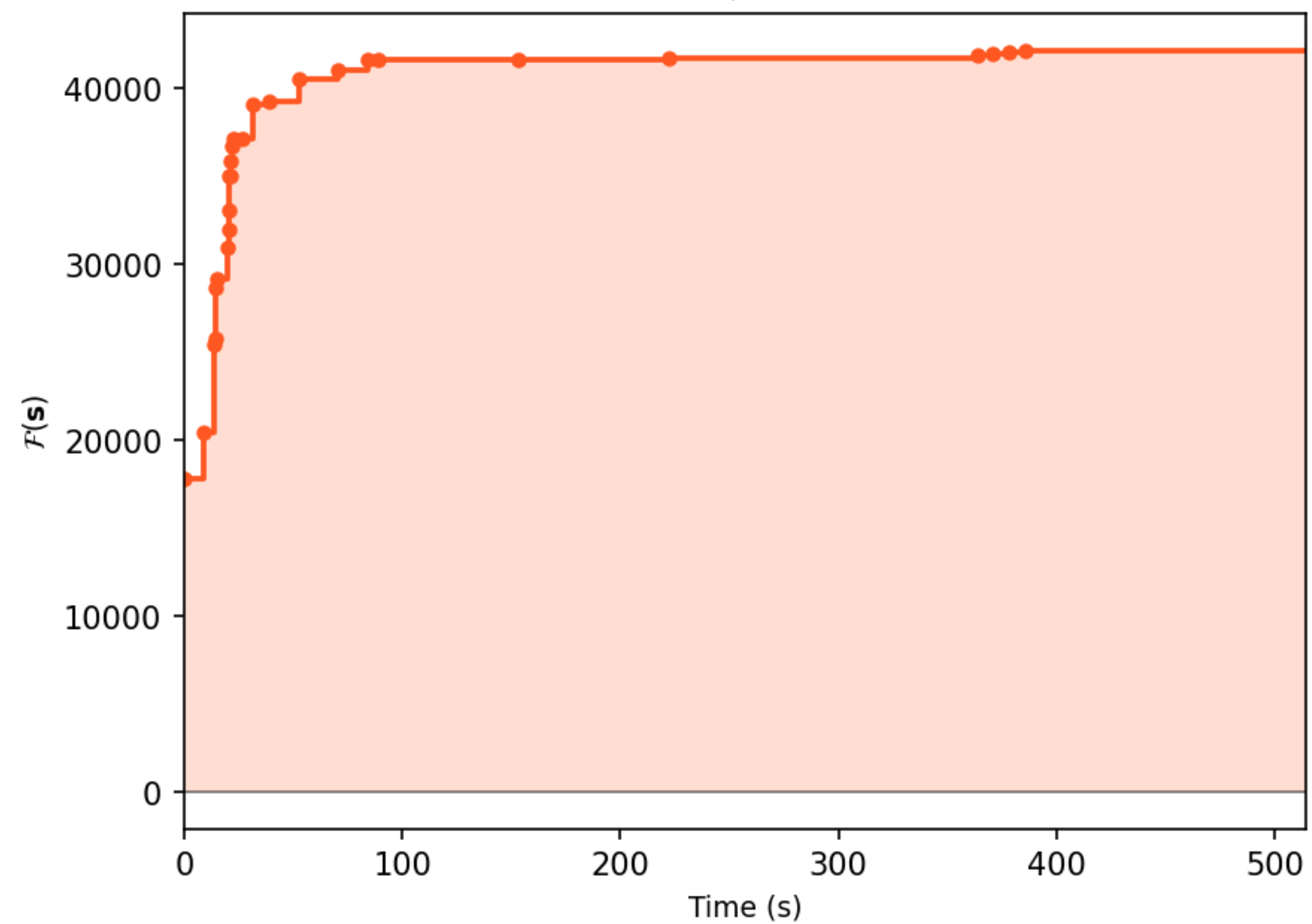
Variable=15800, clauses=48478
