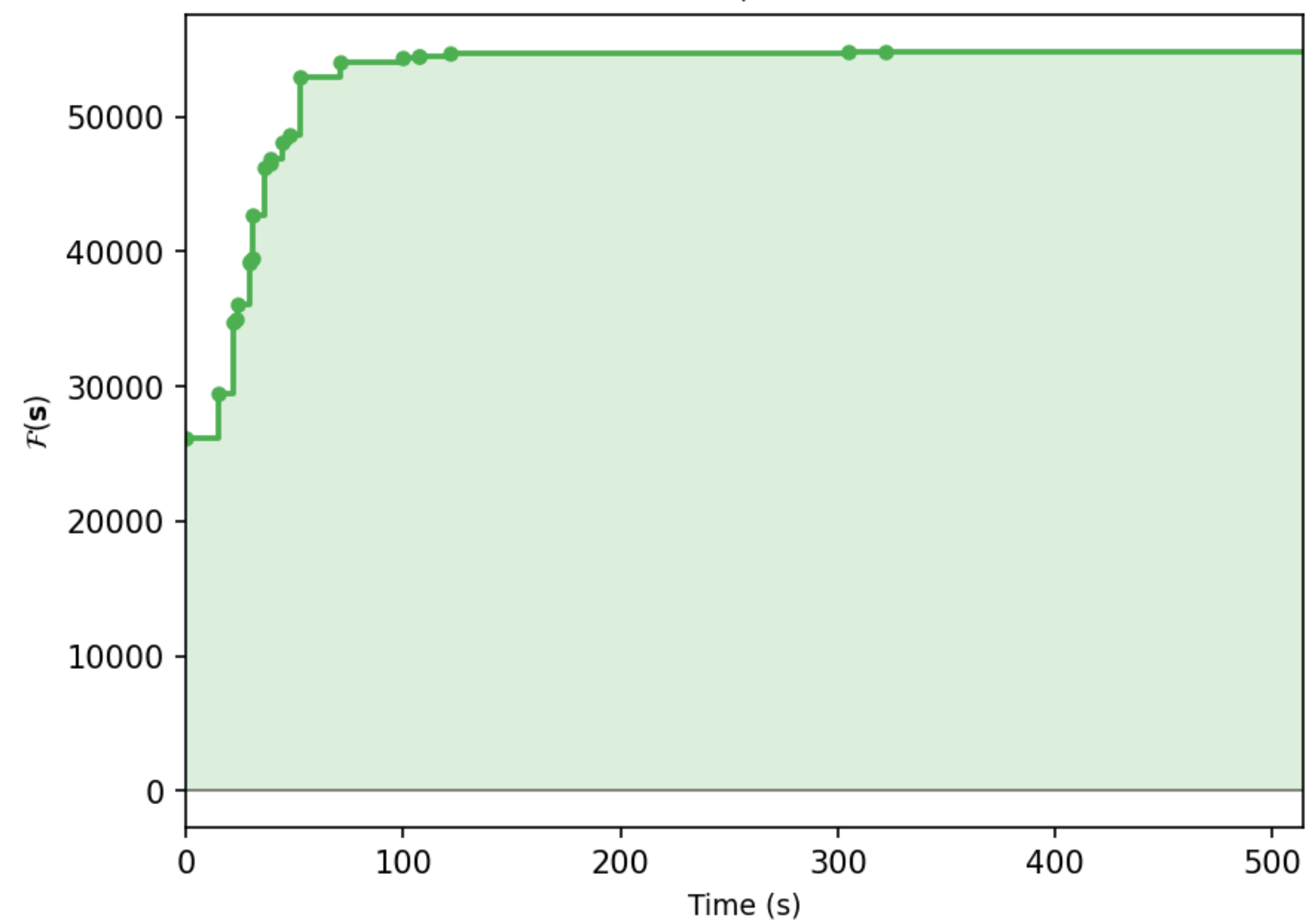
Variable=11850, clauses=36296
