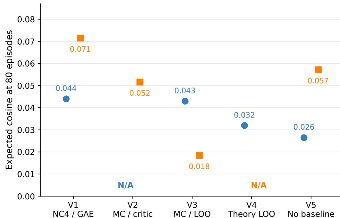
Expected training-batch gradient cosine
