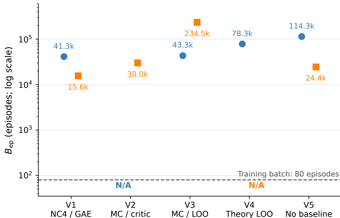
Critical batch size in episodes
