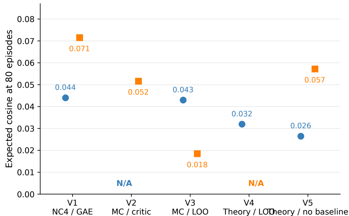
Expected training-batch gradient cosine
