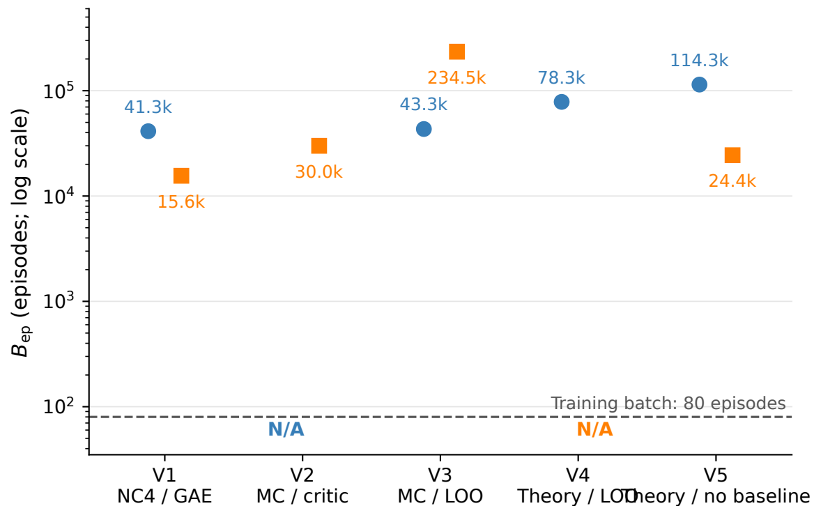
Critical batch size in episodes
