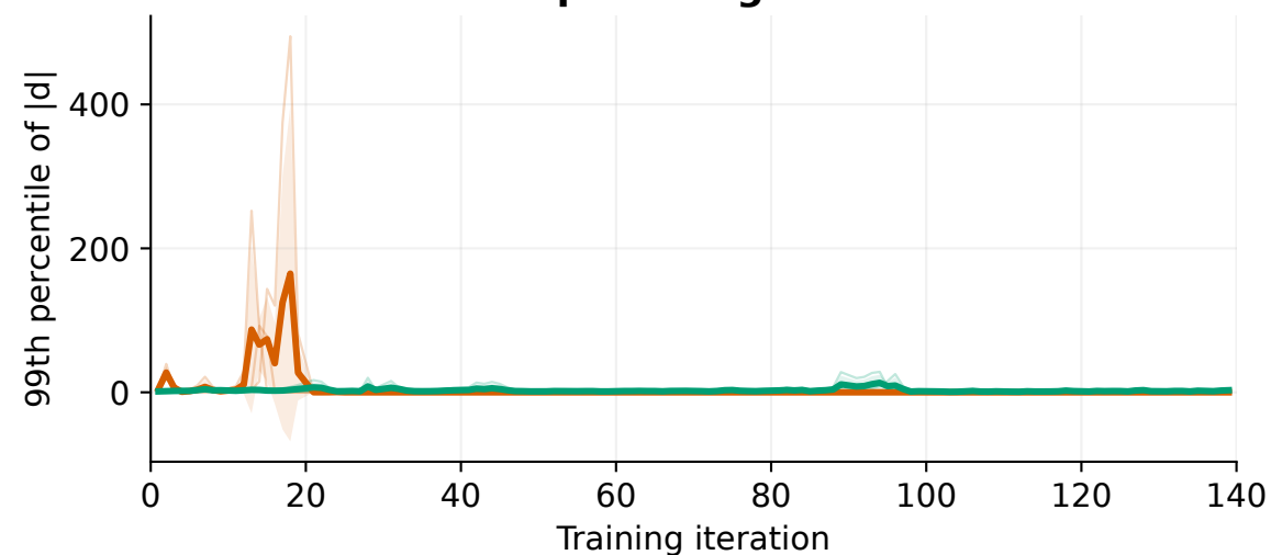
Post-update log-ratio tail
