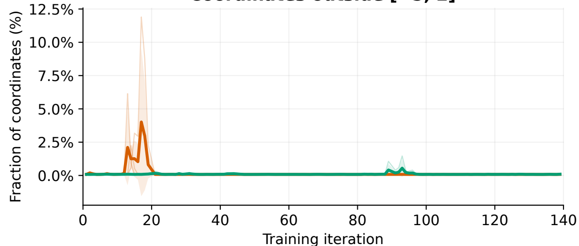
Coordinates outside [-5, 2]
