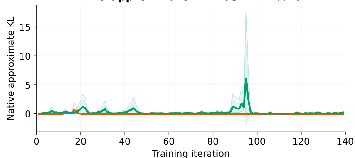
DPPO approximate KL · last minibatch
