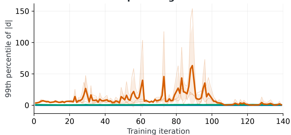
Post-update log-ratio tail
