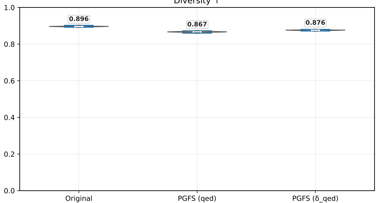
Internal test (Bi pool) — PGFS uses max-QED per episode; Original = start molecules
