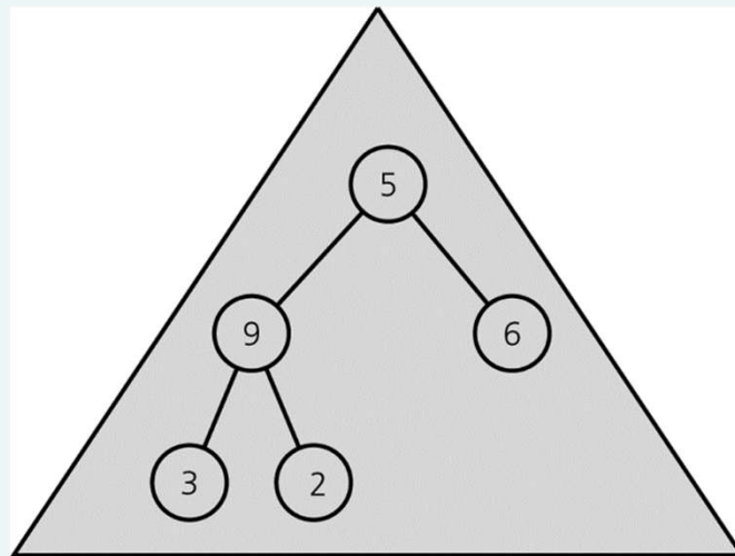
First semiheap passed to heapRebuild
