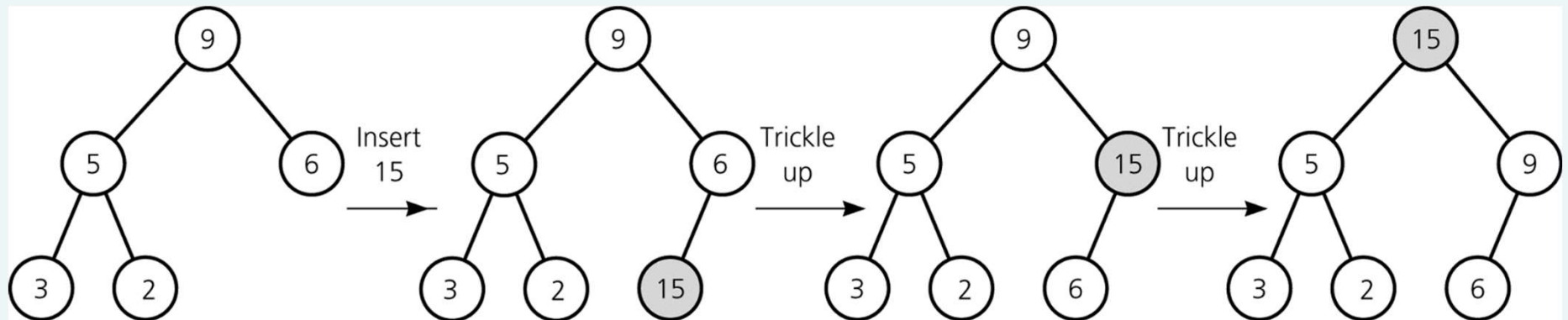
Insertion into a heap
