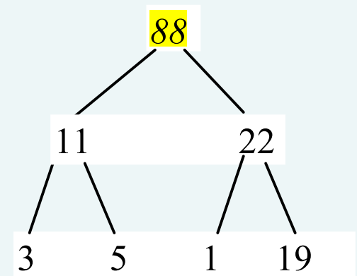
(b) After swapping 88 with 22
