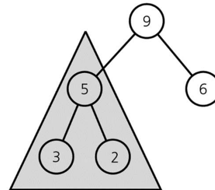
Second semiheap passed to heapRebuild
