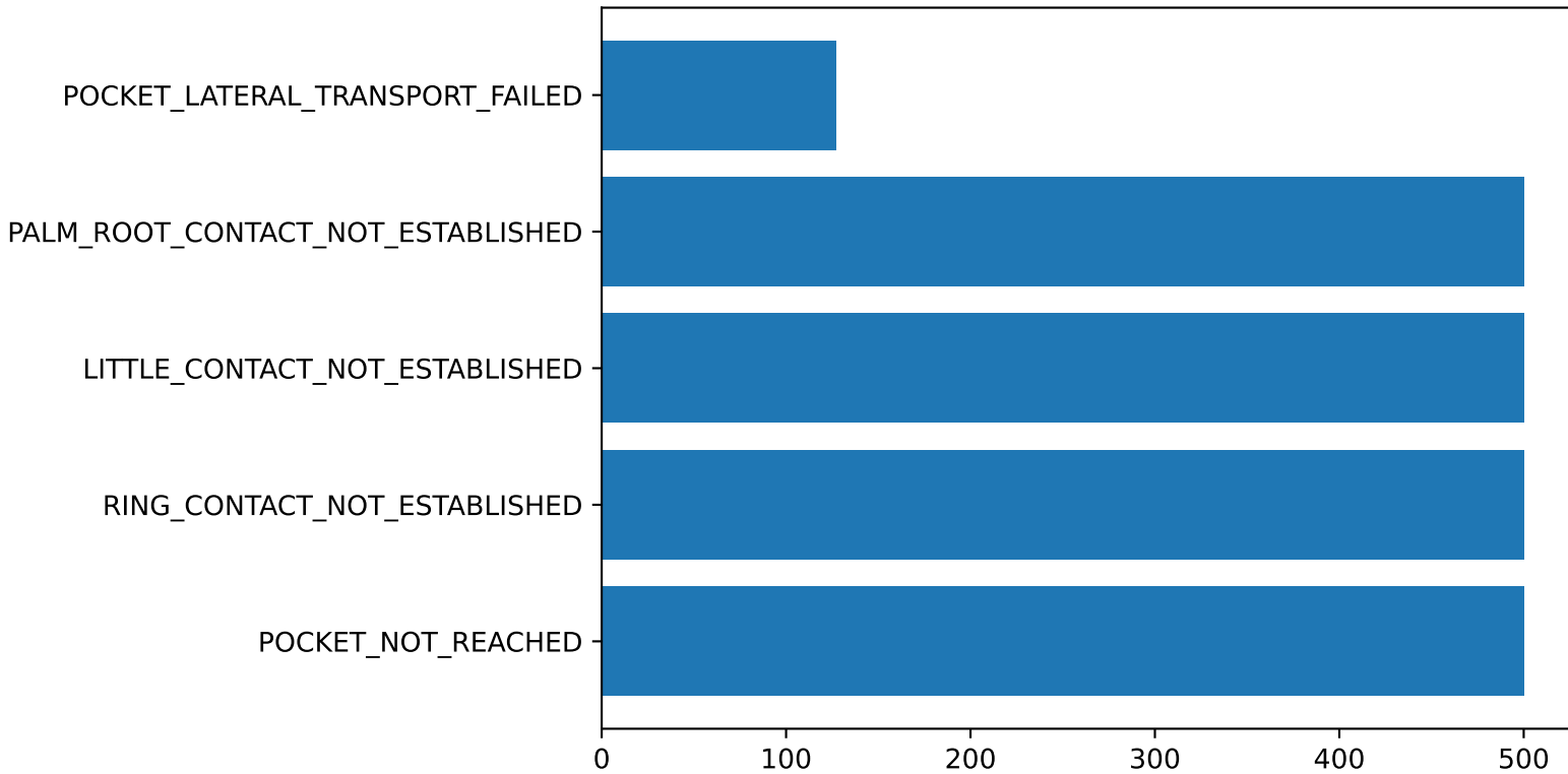
Protocol failure taxonomy
