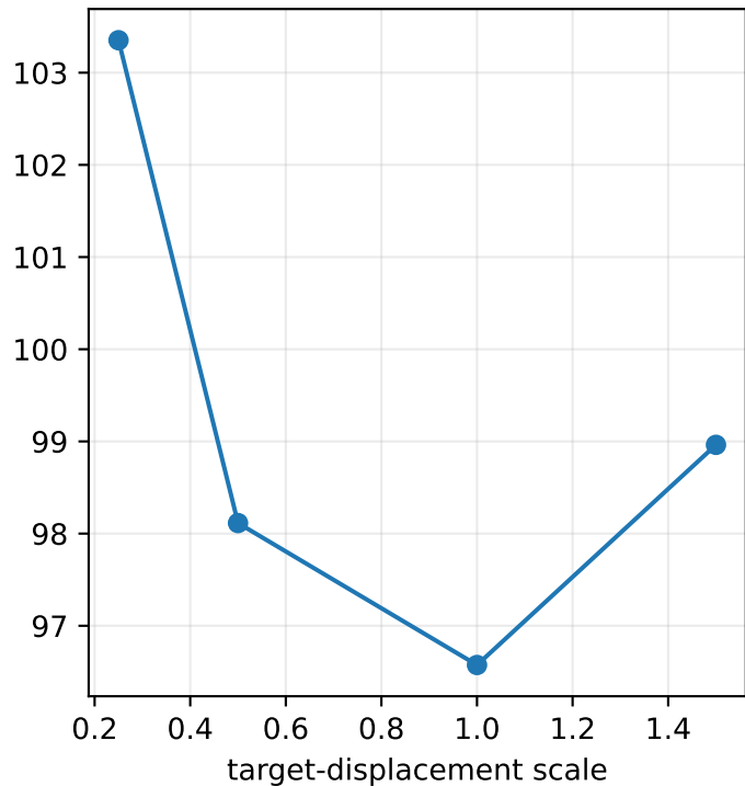
p95 max object acceleration (m/s 2 )
