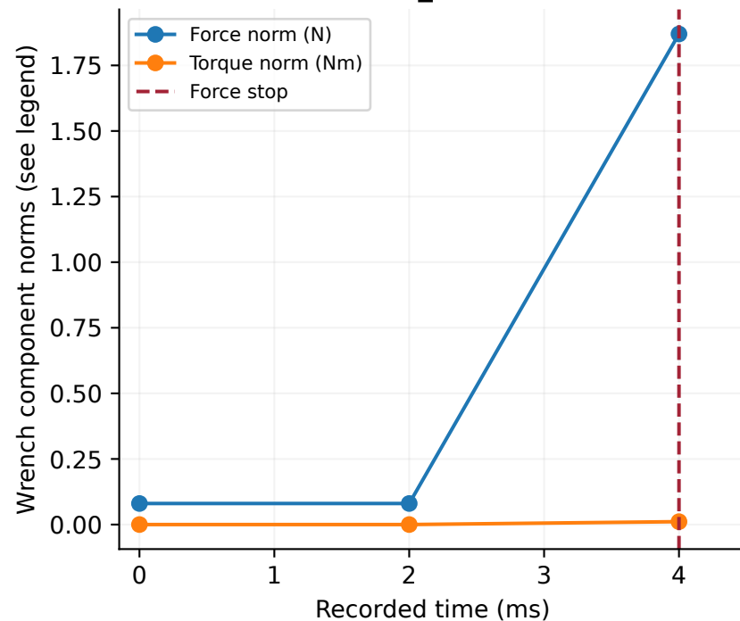
TC10_IMP99
