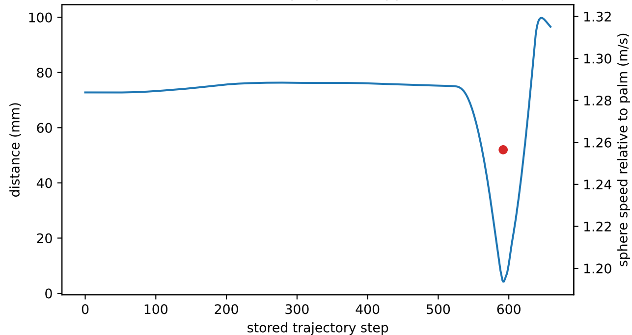
Phase 3C-0.8 4.226-mm fly-by is unsupported and rejected
