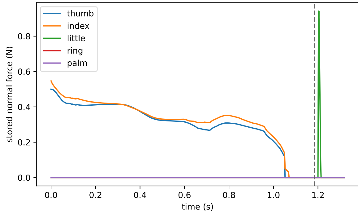
Best trajectory stored contact forces
