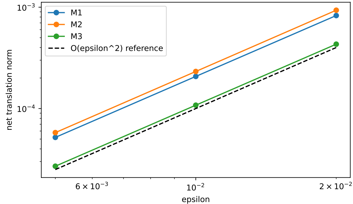
Kinematic cyclic bracket validation
