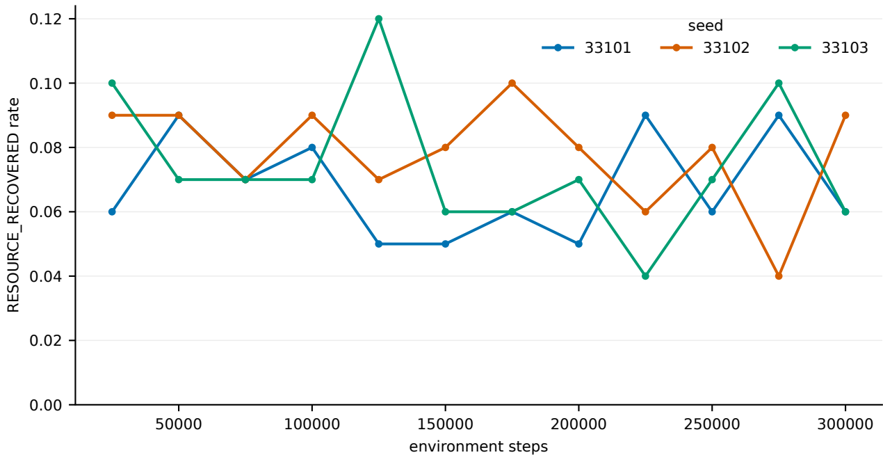
Held-out validation resource recovery
