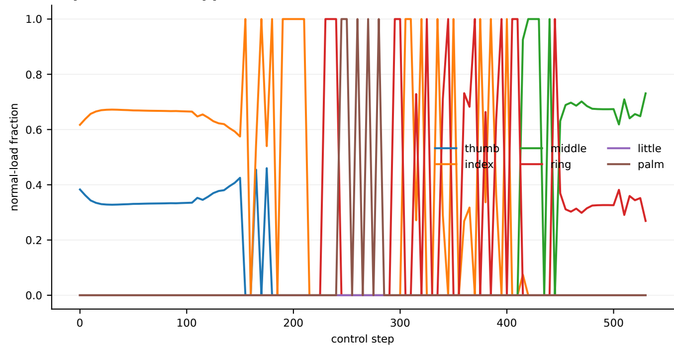
Representative support-load evolution
