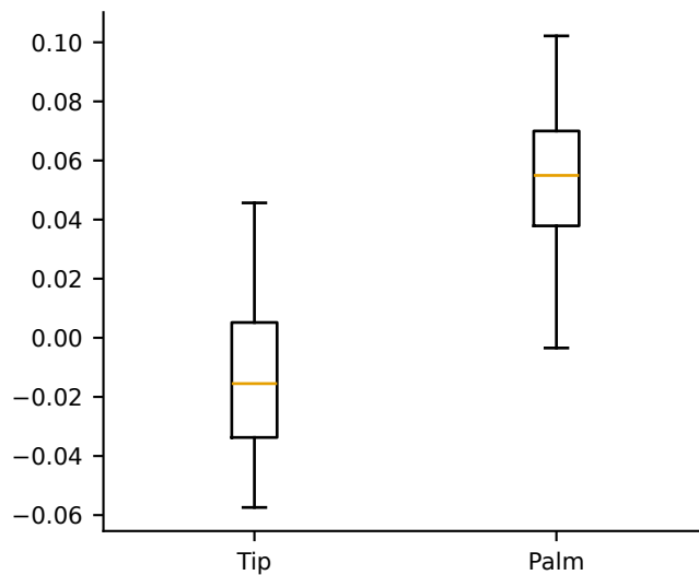
minimum joint margin rad
