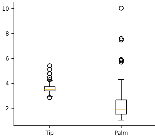
minimum joint margin rad
