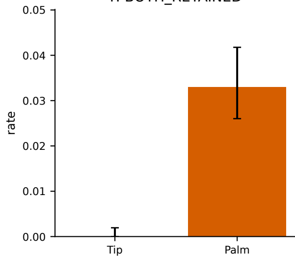
F. BOTH_RETAINED
