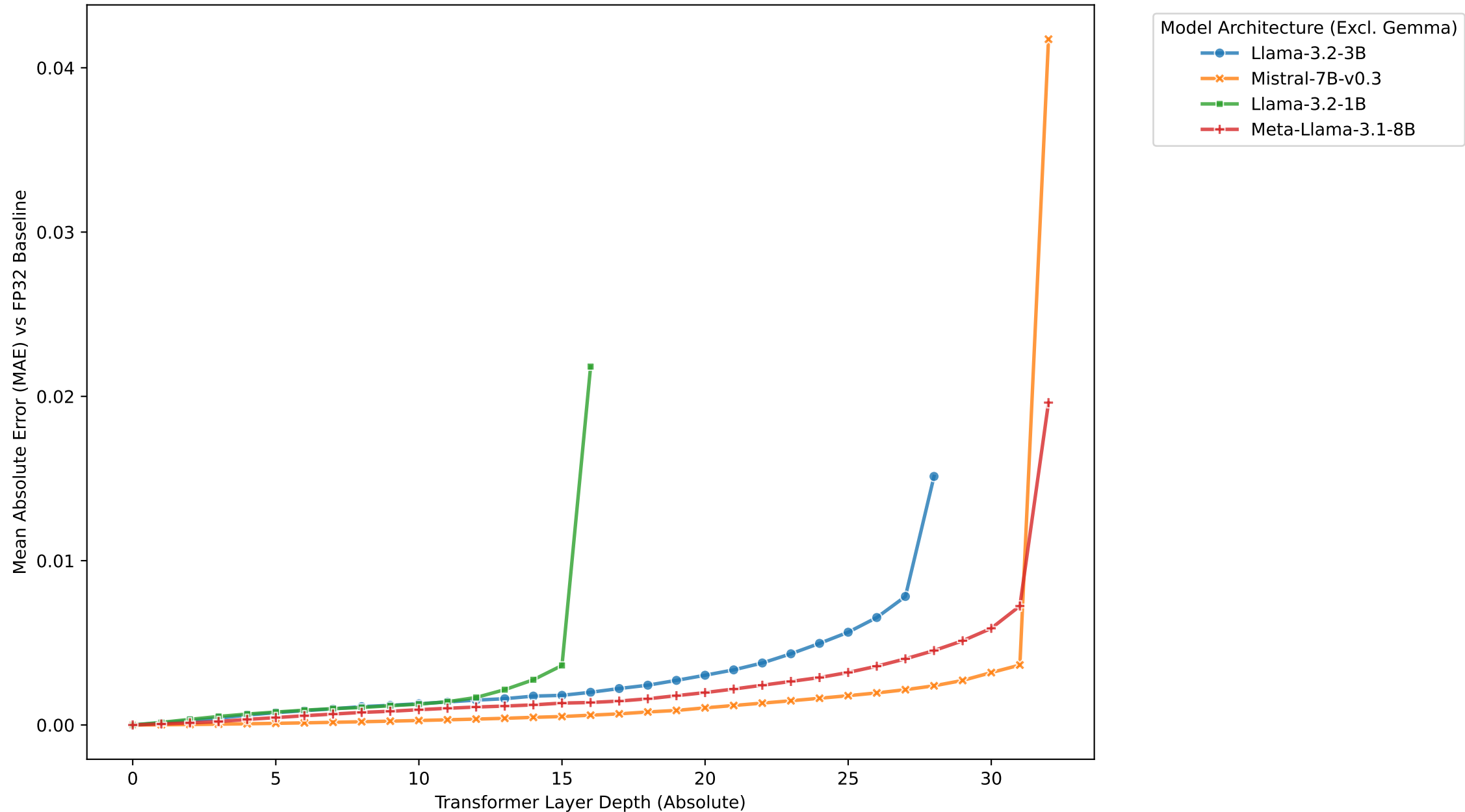
[CMMLU] Layer-wise Error Trend: FP32 vs BF16
