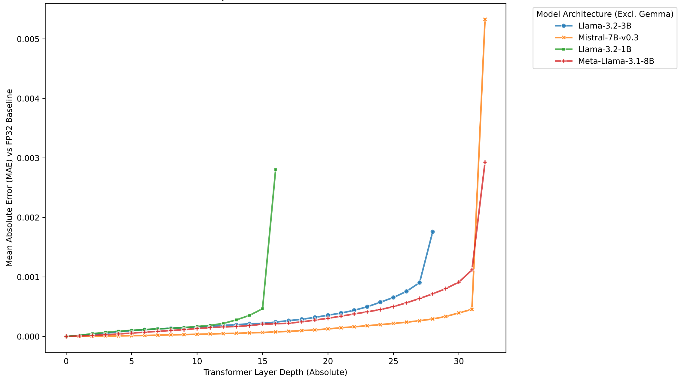
[CMMLU] Layer-wise Error Trend: FP32 vs FP16
