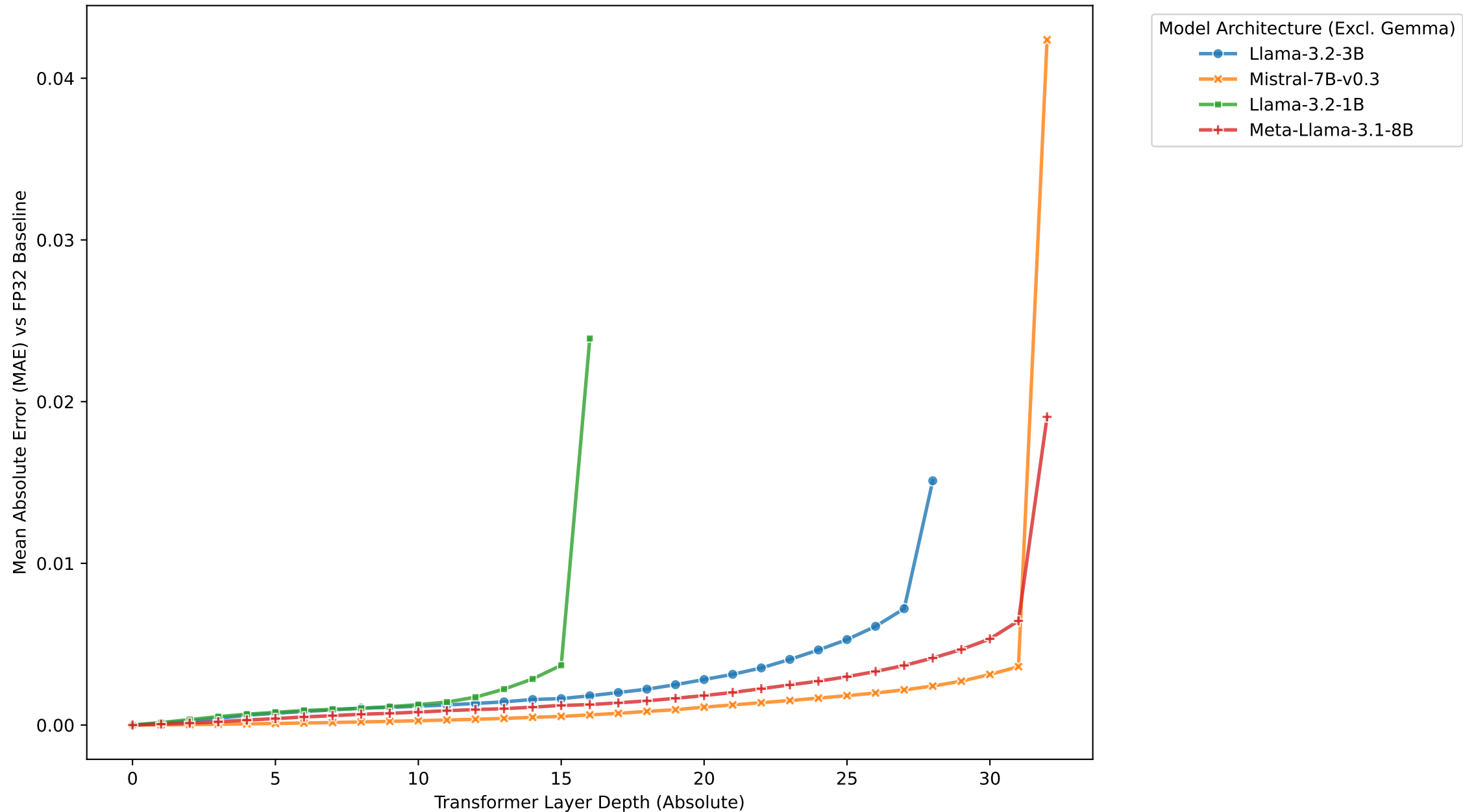
[HUMANEVAL] Layer-wise Error Trend: FP32 vs BF16
