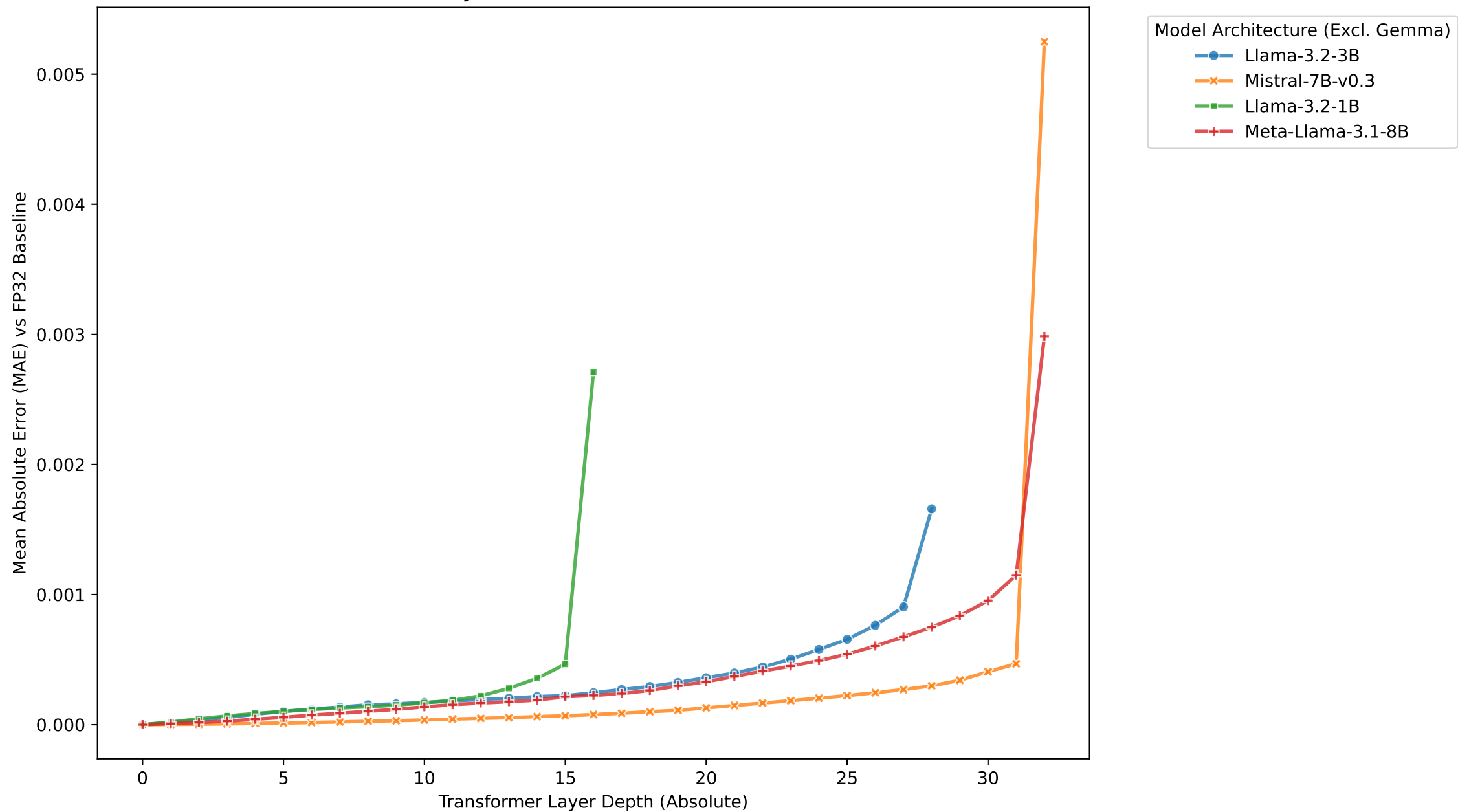
[PIQA] Layer-wise Error Trend: FP32 vs FP16
