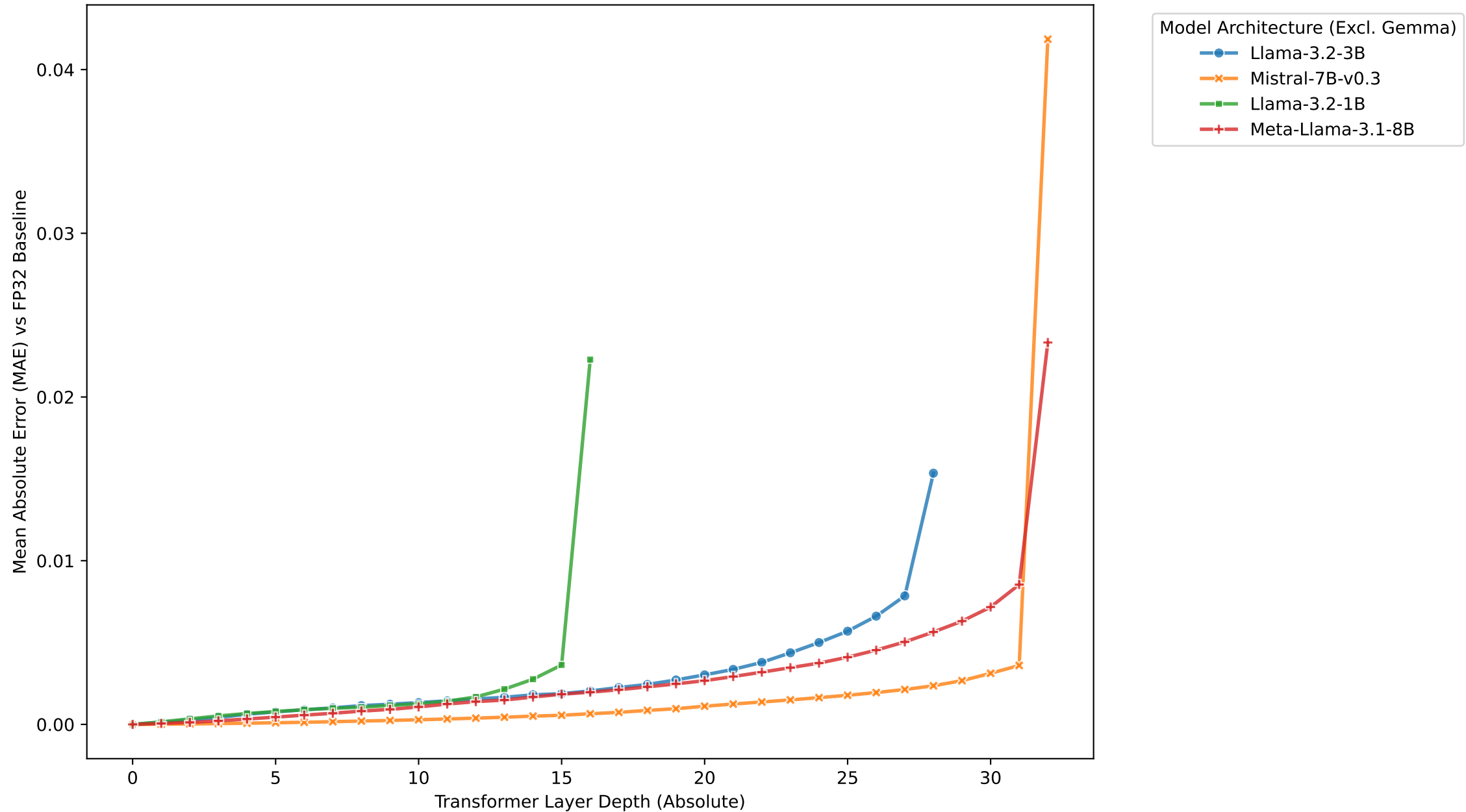
[GSM8K] Layer-wise Error Trend: FP32 vs BF16
