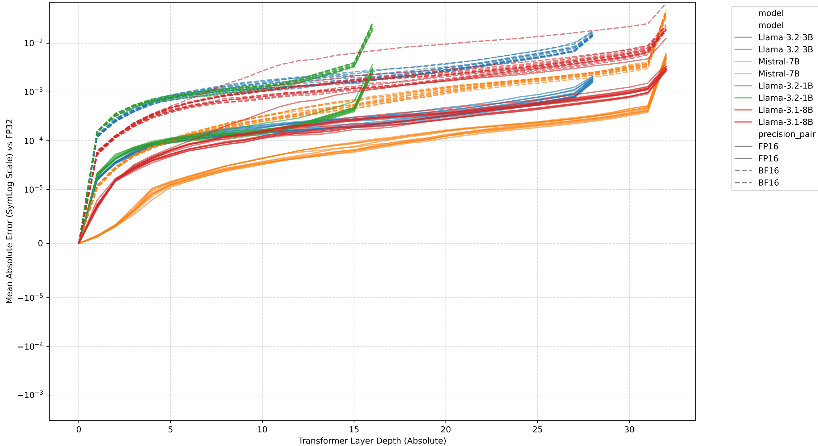
[GSM8K] ALL Cases: Individual Layer MAE Trends (BF16 & FP16 vs FP32)
