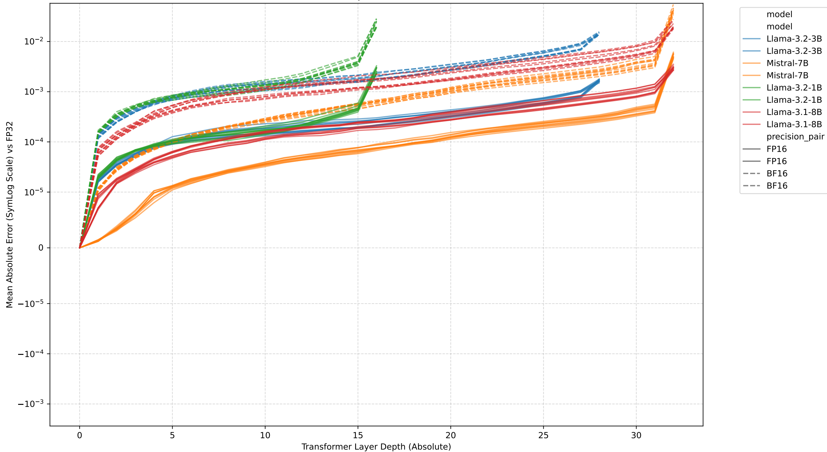
[PIQA] ALL Cases: Individual Layer MAE Trends (BF16 & FP16 vs FP32)
