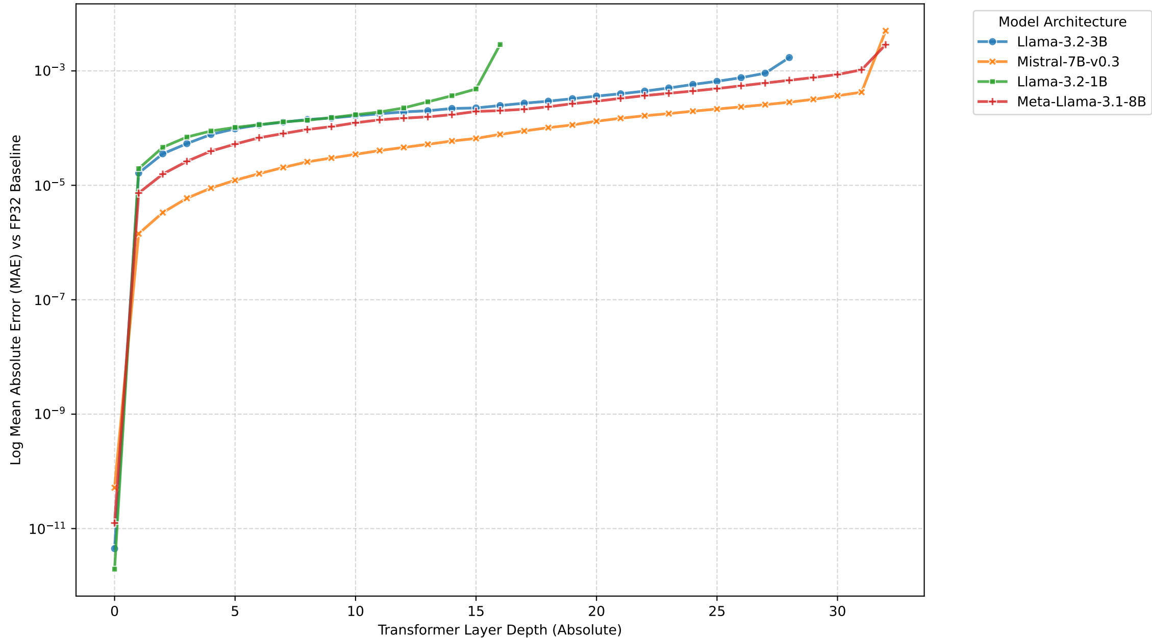
[CMMLU] DIVERGENT Only Log-Scale Layer-wise Error Trend: FP32 vs FP16
