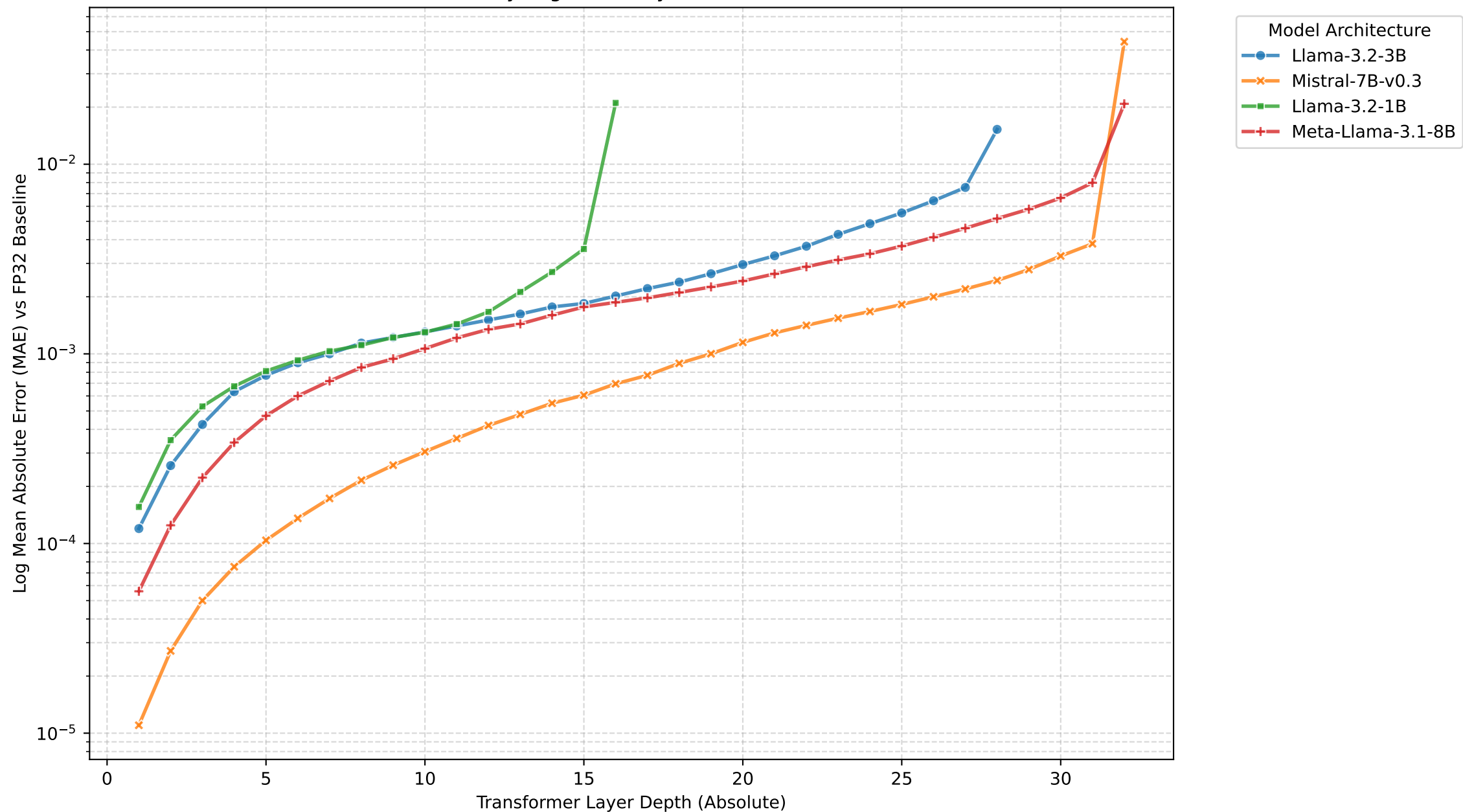
[GSM8K] DIVERGENT Only Log-Scale Layer-wise Error Trend: FP32 vs BF16
