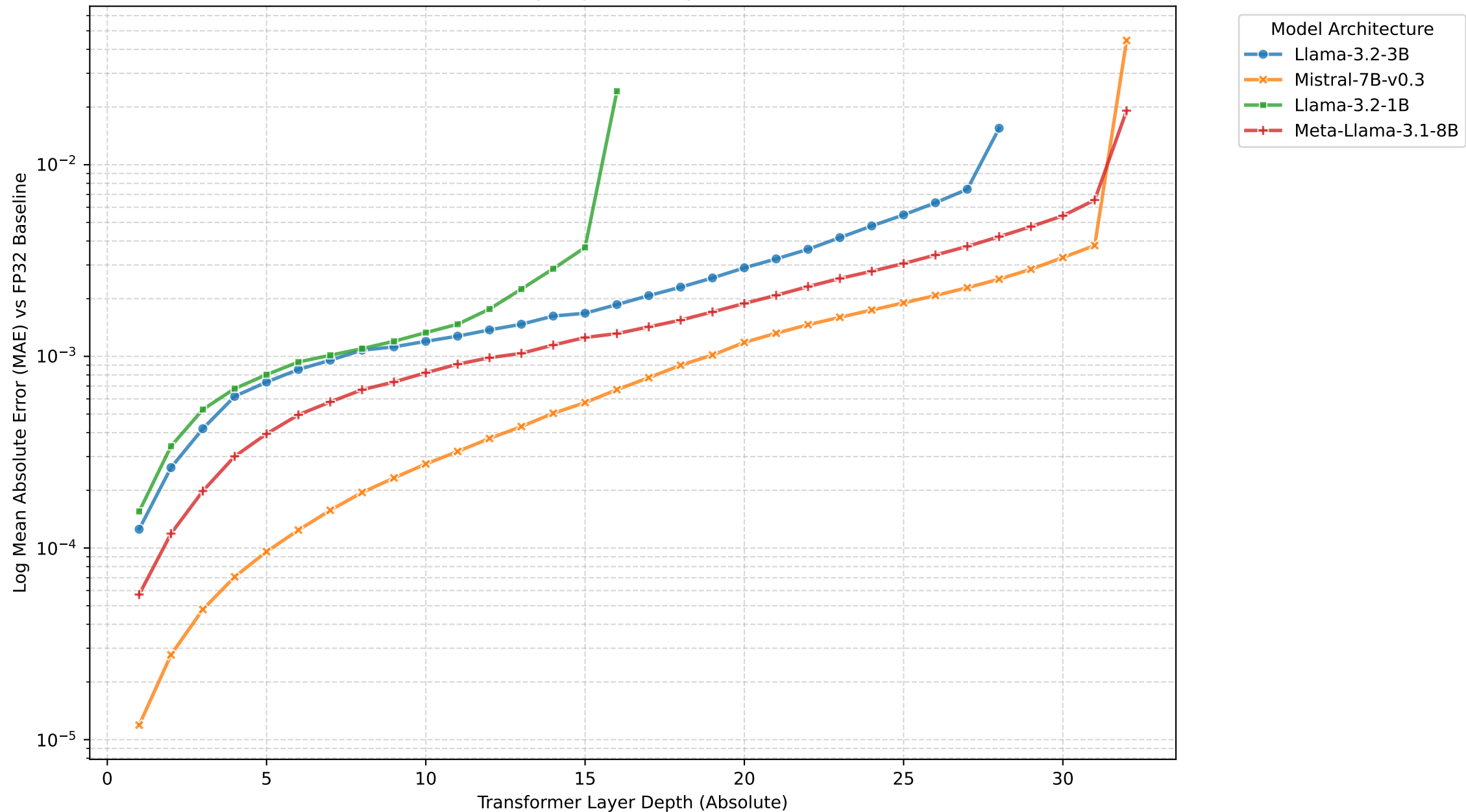
[HUMANEVAL] DIVERGENT Only Log-Scale Layer-wise Error Trend: FP32 vs BF16
