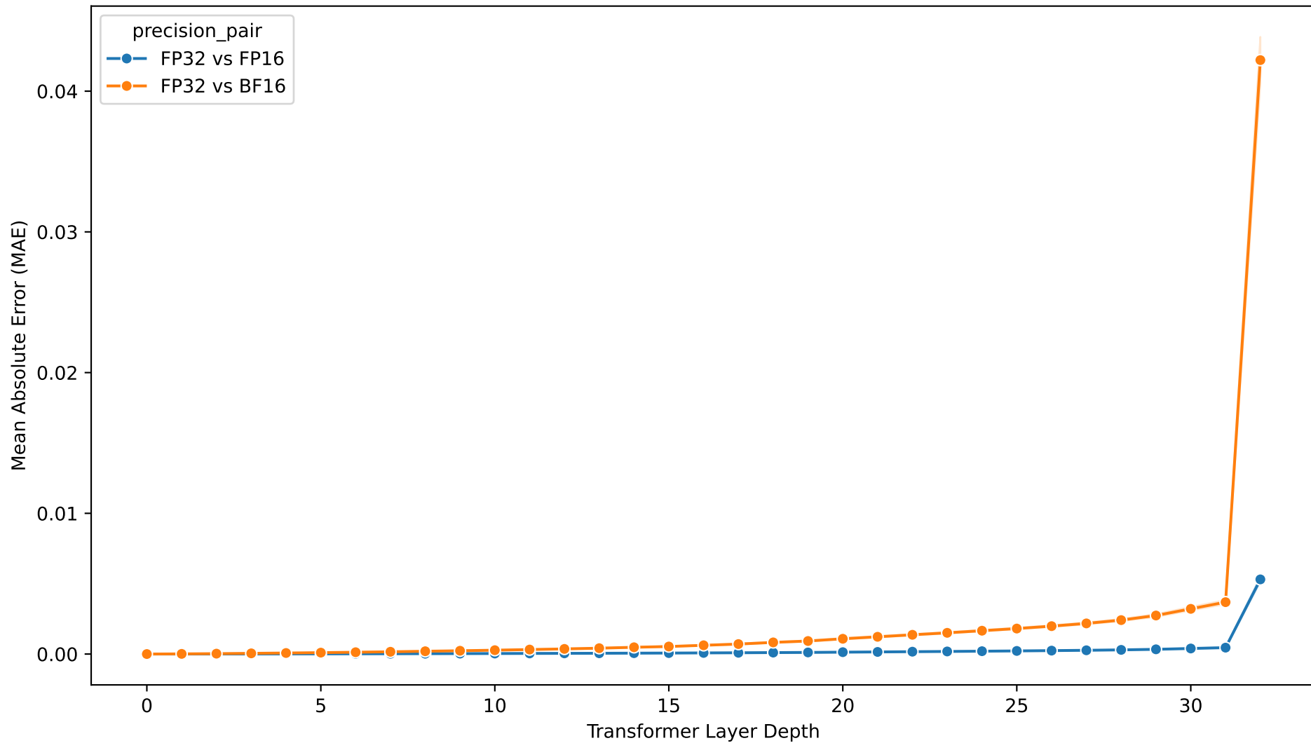
Mistral-7B-v0.3 - Layer-wise Hidden-State Mean Absolute Error
