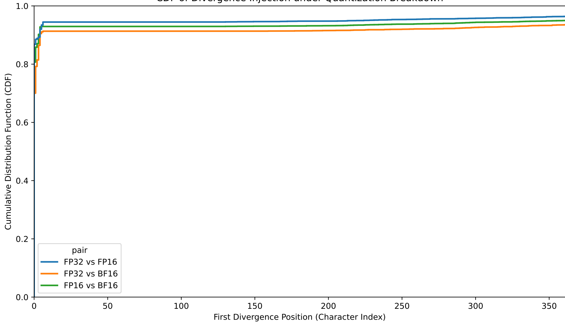
CDF of Divergence Injection under Quantization Breakdown
