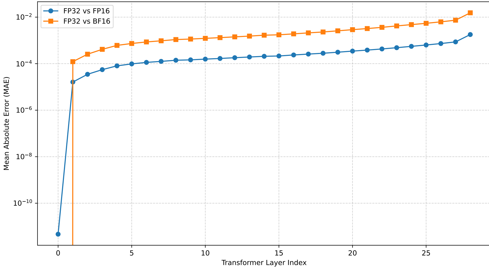
Layer-wise Hidden-State MAE (Llama-3.2-3B under Quantization)
