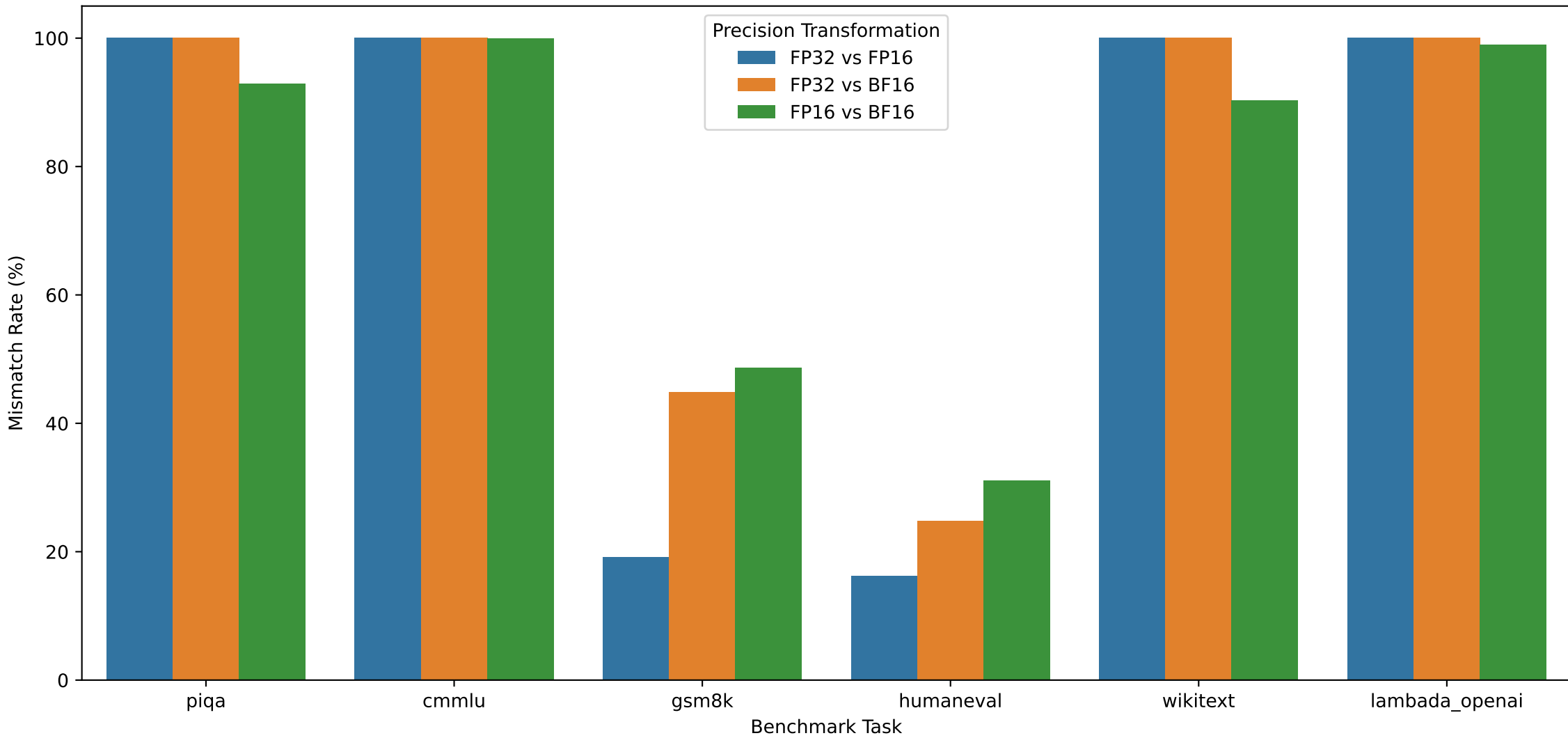
Sequence Mismatch Rate by Benchmark under Precision Variance
