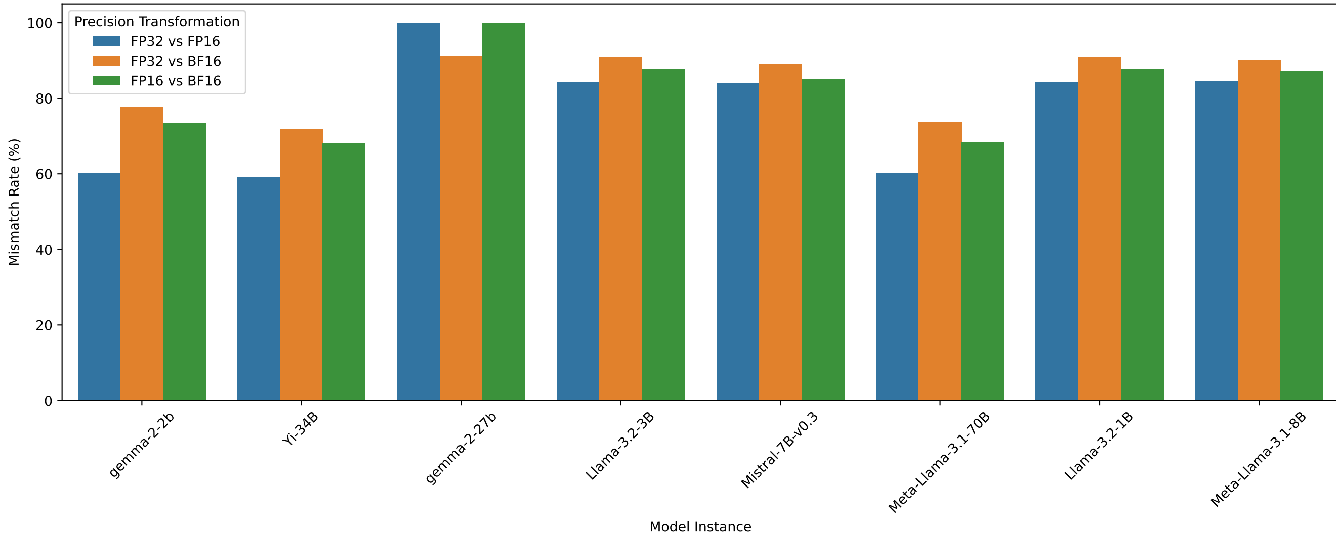
Sequence Mismatch Rate by Model under Precision Variance
