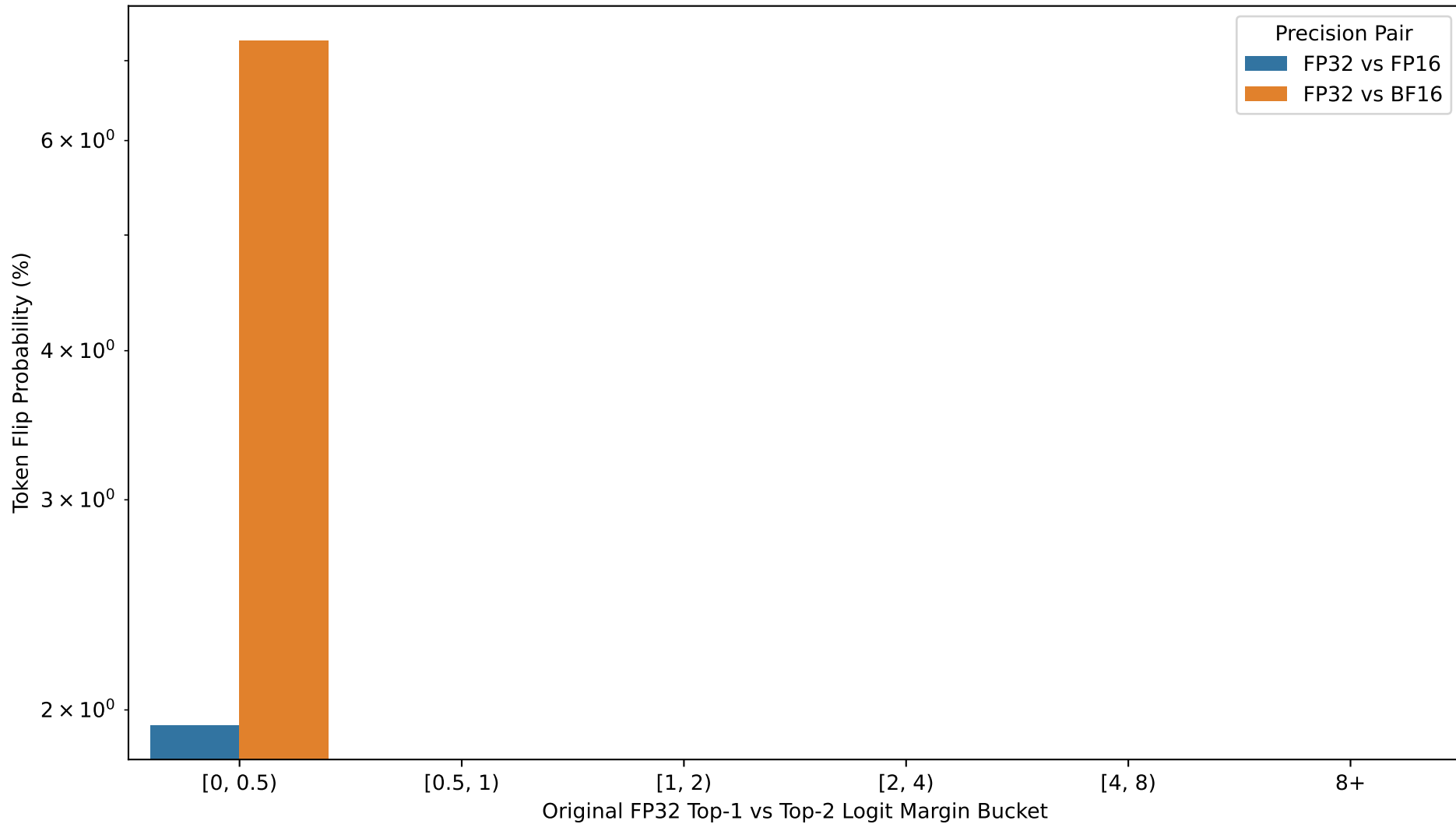
Token Flip Probability vs Logit Margin
