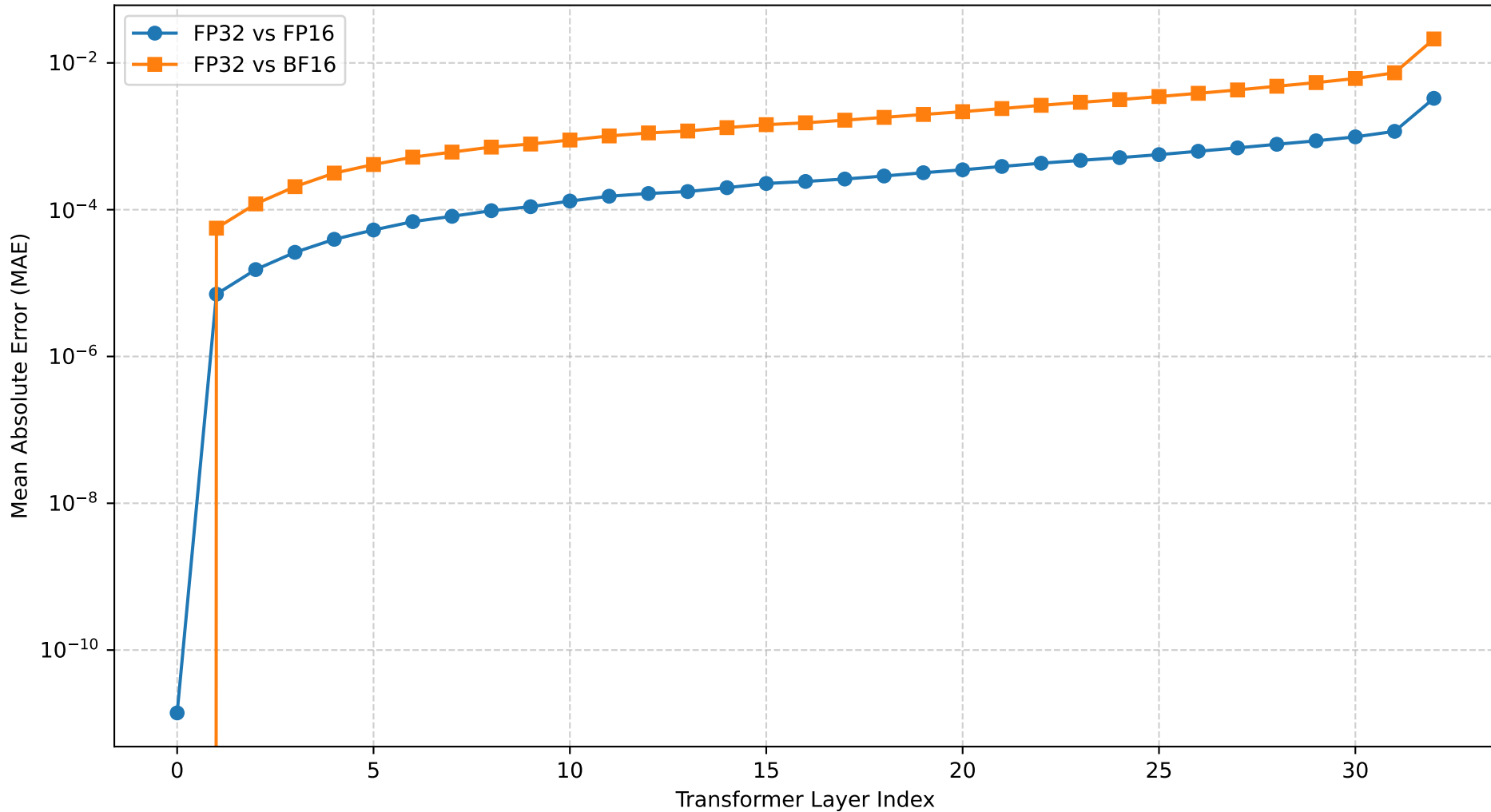
Layer-wise Hidden-State MAE (Meta-Llama-3.1-8B under Quantization)
