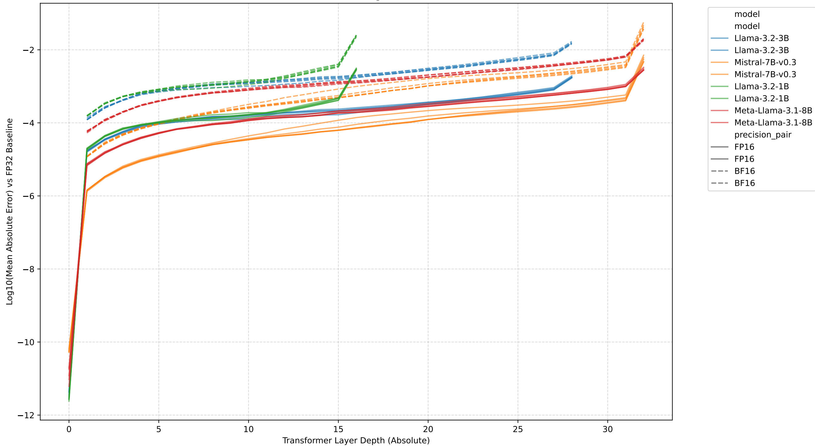
[HUMANEVAL] DIVERGENT Cases: Individual Log10 MAE Trends (BF16 & FP16 vs FP32)
