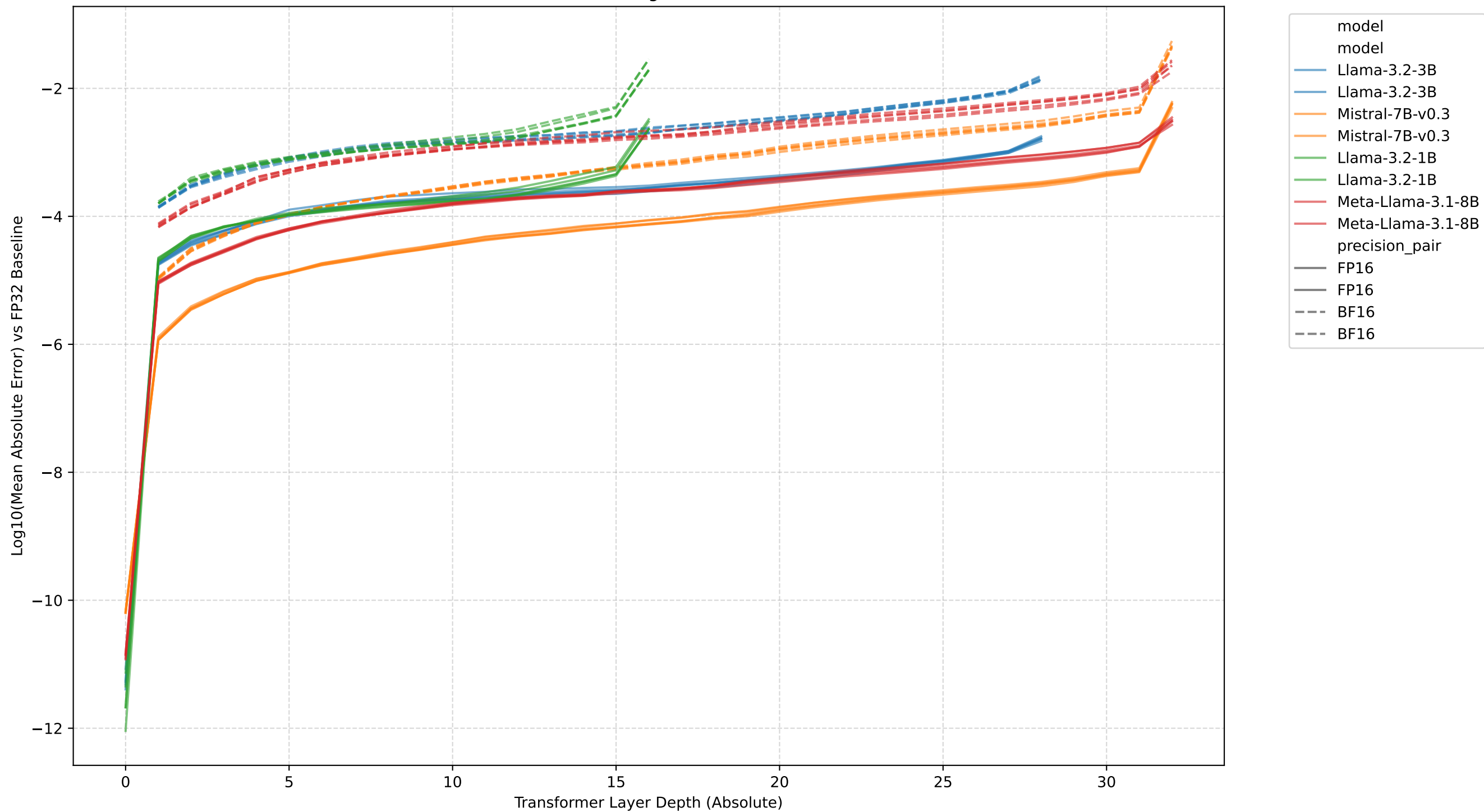
[PIQA] DIVERGENT Cases: Individual Log10 MAE Trends (BF16 & FP16 vs FP32)
