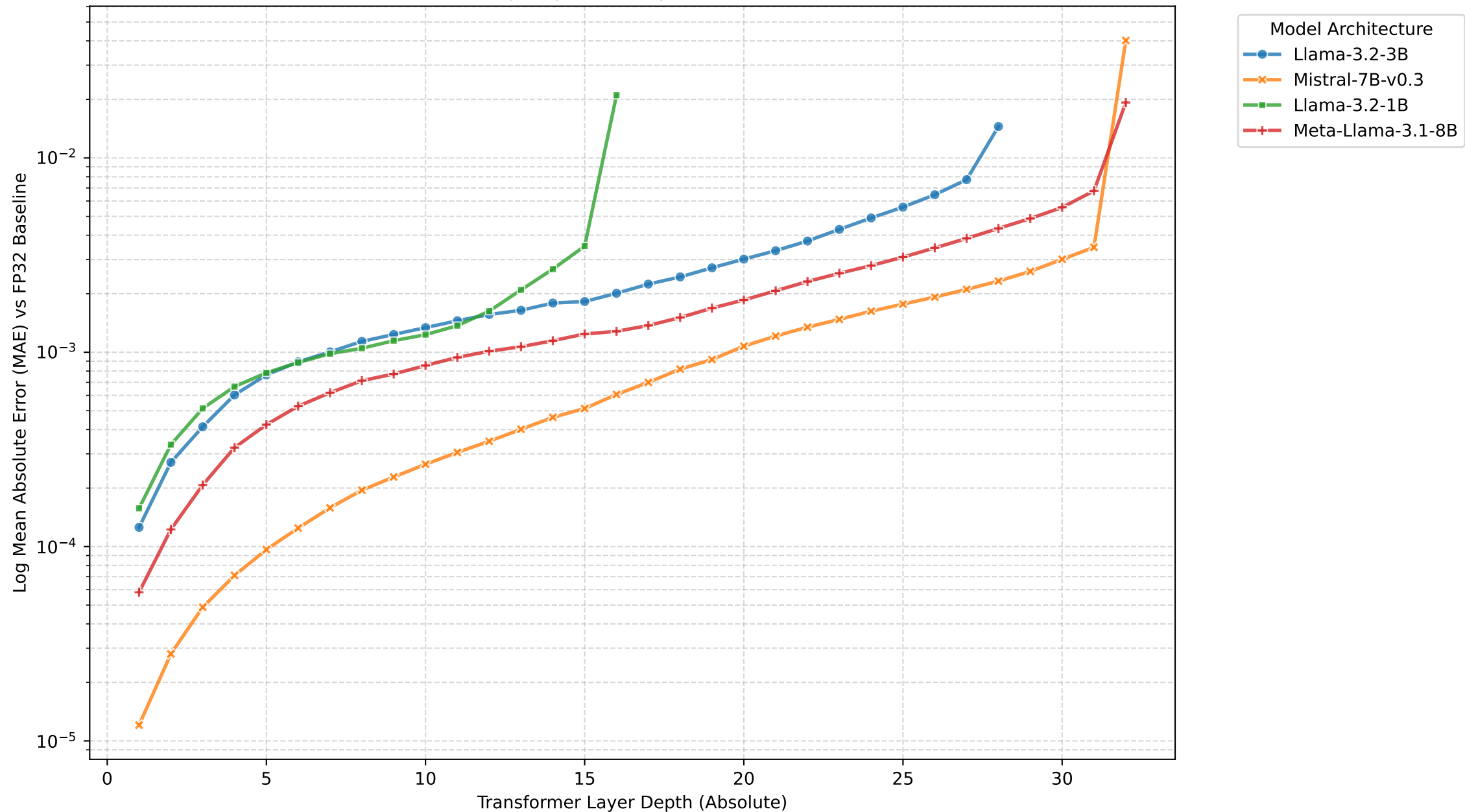
[CMMLU] DIVERGENT Only Log-Scale Layer-wise Error Trend: FP32 vs BF16
