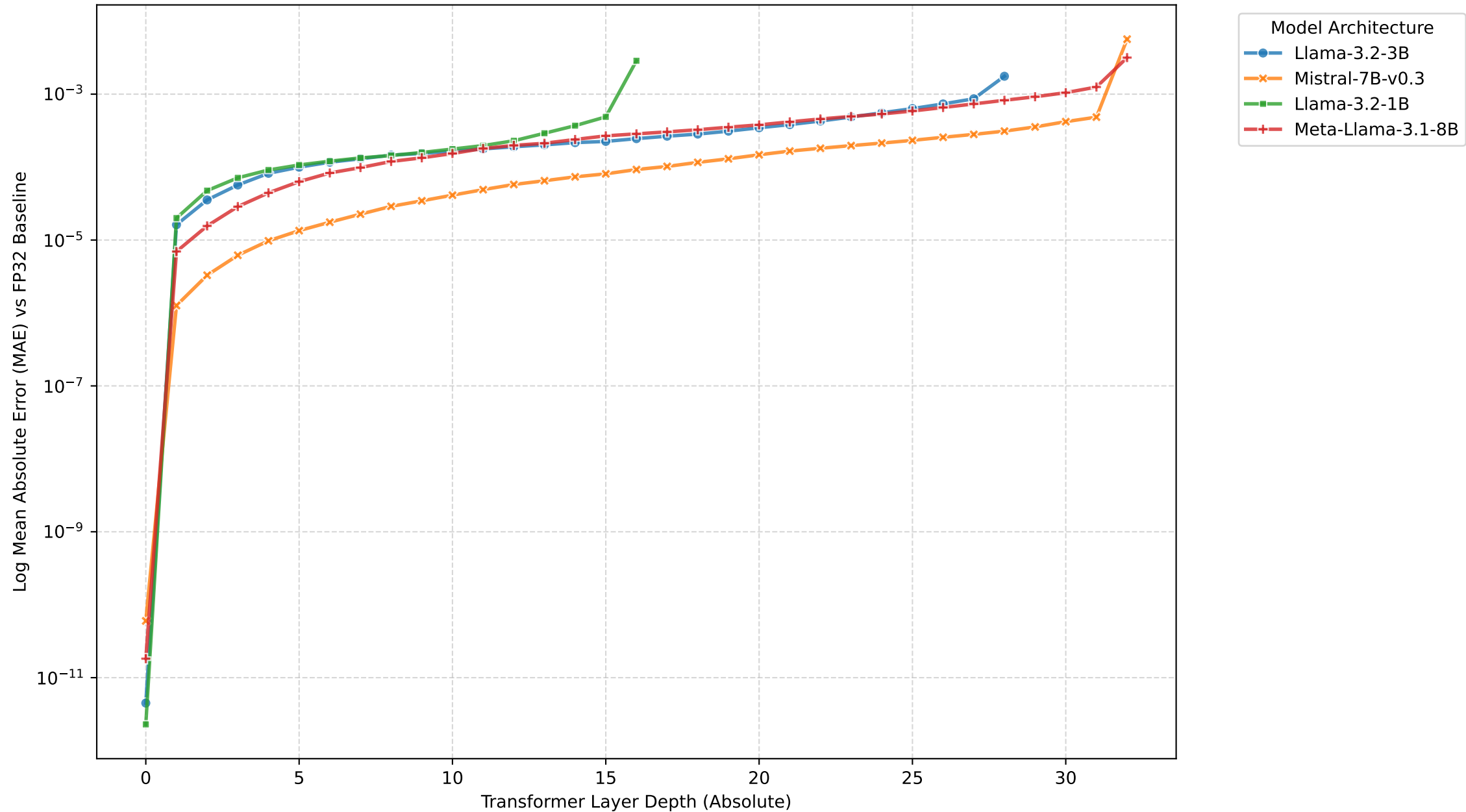
[GSM8K] DIVERGENT Only Log-Scale Layer-wise Error Trend: FP32 vs FP16
