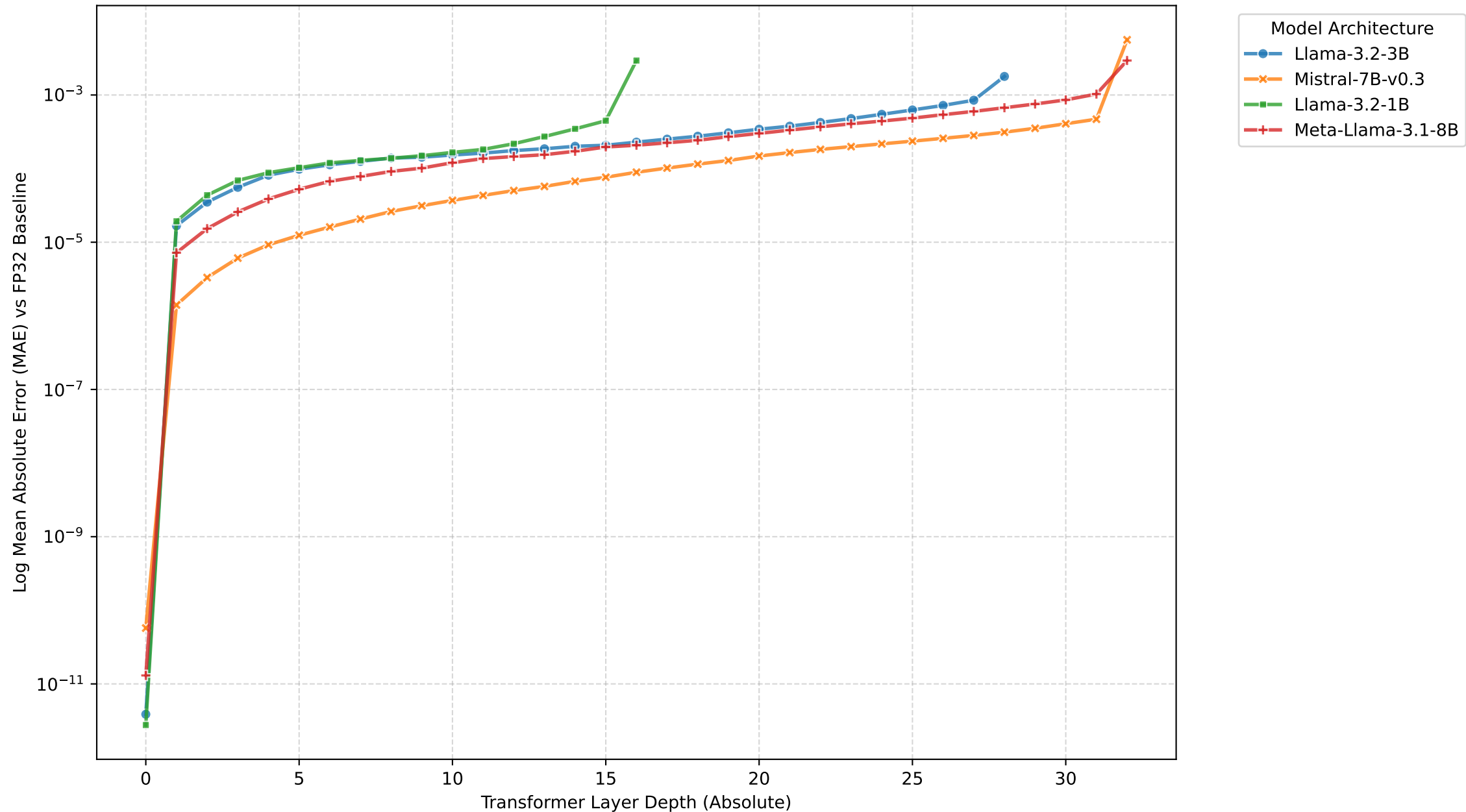
[HUMANEVAL] DIVERGENT Only Log-Scale Layer-wise Error Trend: FP32 vs FP16
