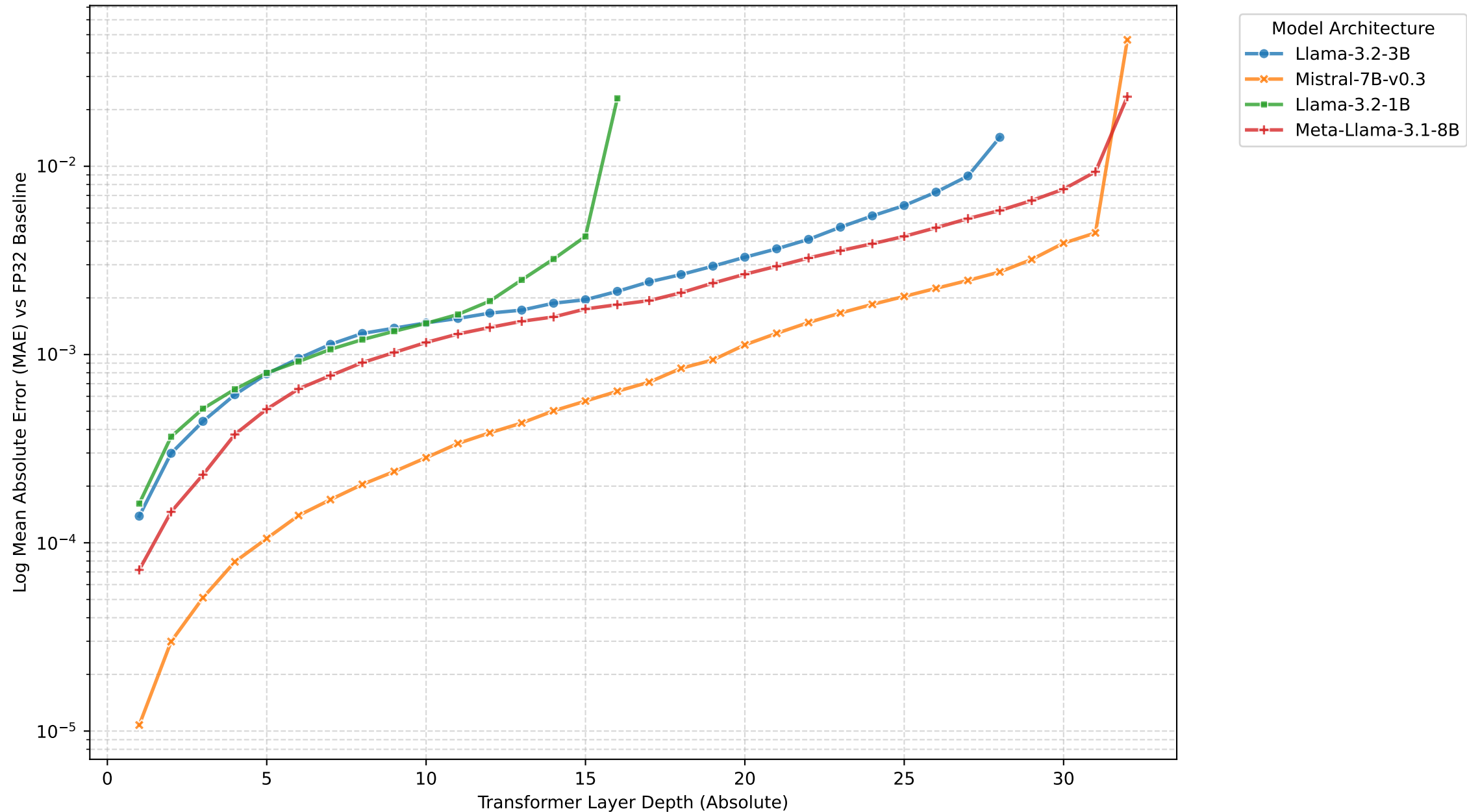
[PIQA] DIVERGENT Only Log-Scale Layer-wise Error Trend: FP32 vs BF16
