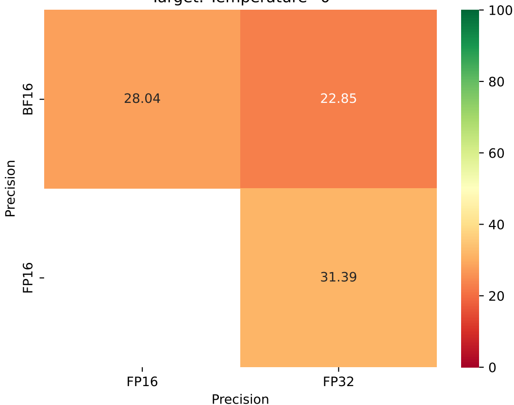
Mistral-7B-v0.3 - Precision Consistency (%) Target: Temperature=0
