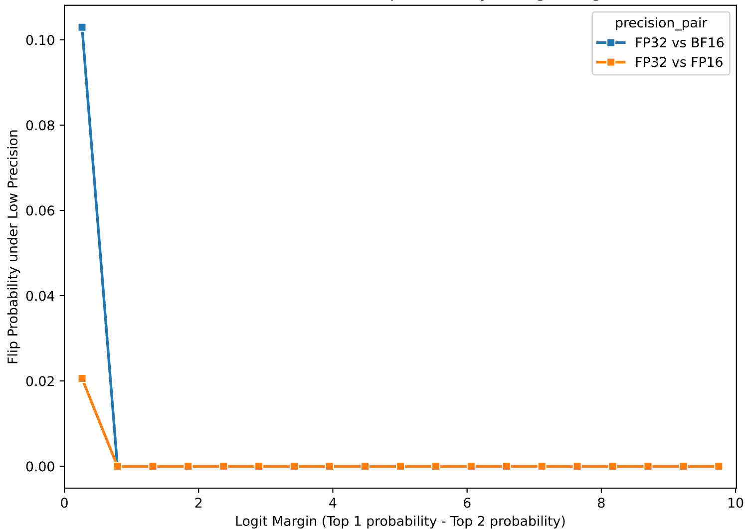
Mistral-7B-v0.3 - Token Flip Probability vs Logit Margin
