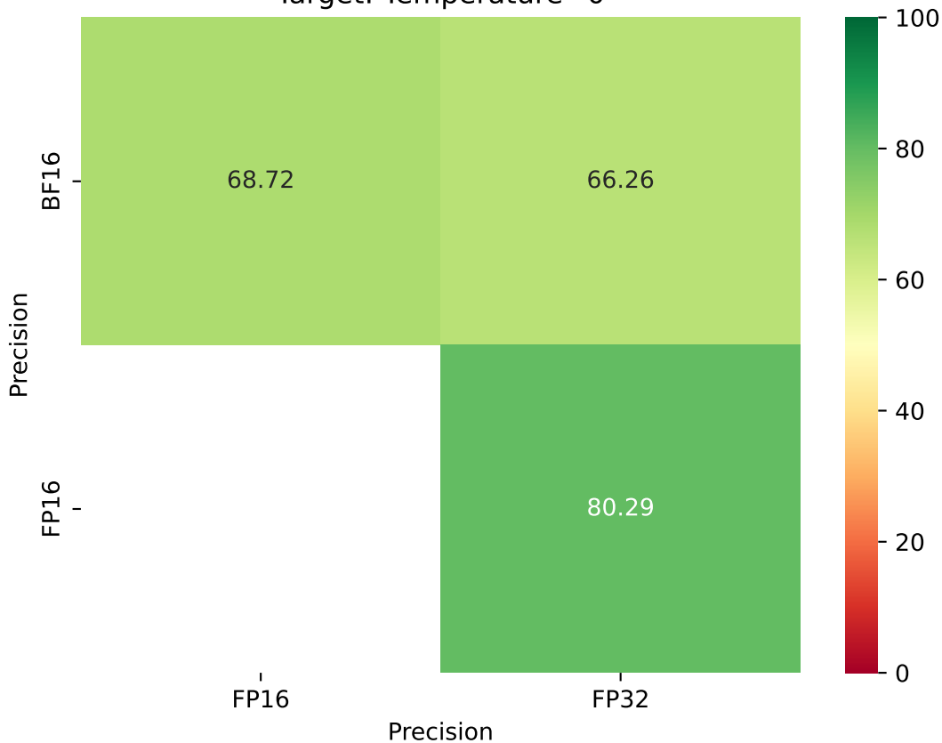
Yi-34B - Precision Consistency (%) Target: Temperature=0
