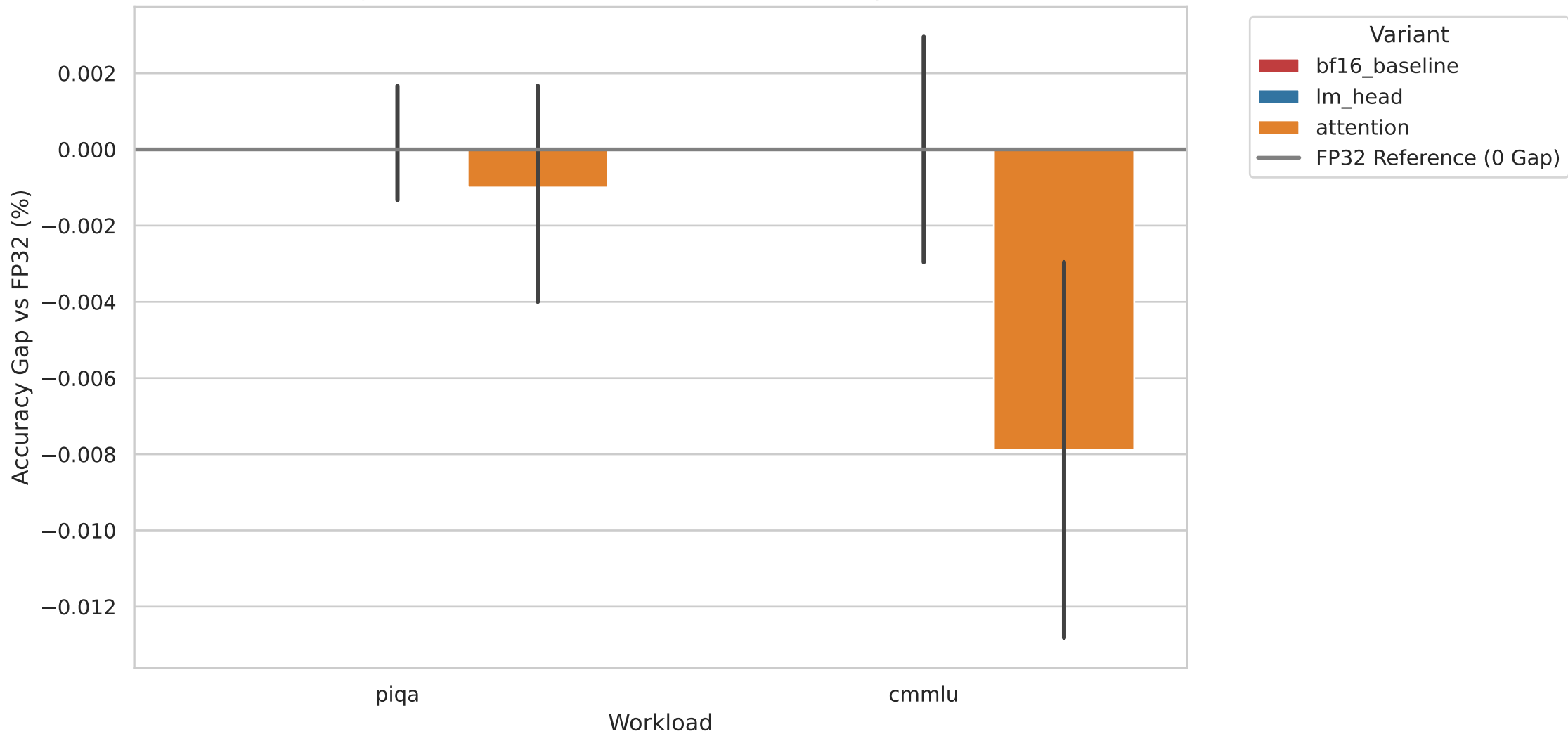
Figure M2. Benchmark Score Deviation Recovery vs FP32
